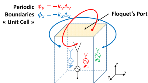
FIGURE 2. Boundary conditions of the computational volume for the IPAA unit cell.
