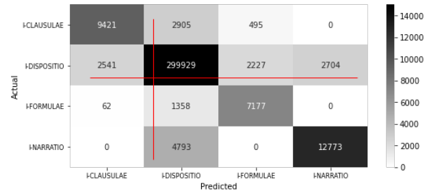
(b) I(inside) labels
