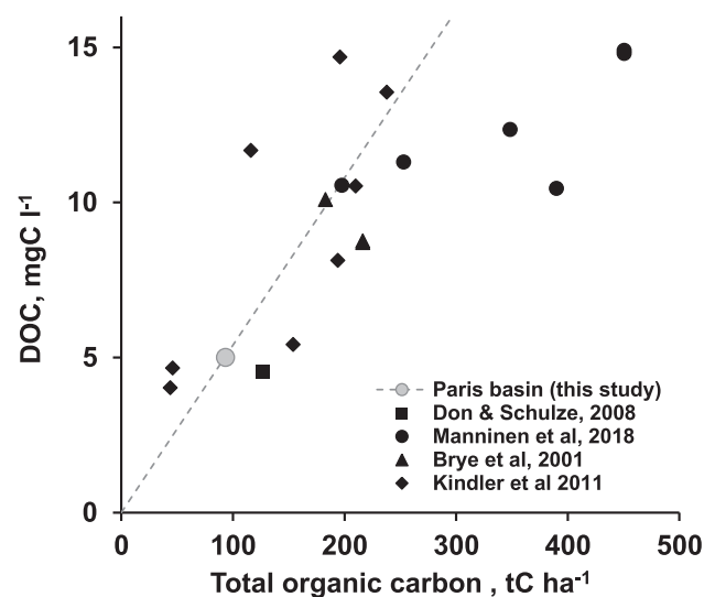
Fig. 8. Relationship between DOC concentrations (flow-weighted leaching) and total soil organic carbon stocks reported in the literature for agricultural and forested watersheds (excluding peat-rich sites). The dashed gray line is equivalent to Eq. (2), assuming an active fraction of 40% of the total soil organic carbon stock.
