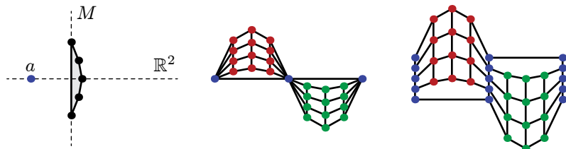
Figure 5. The polygon \Pi (left), the polytopes P_F used to build \tilde{\Xi}(k, l, m) from \Theta(k, l) (center), and a sketch of the Minkowski sum between \Pi and these polytopes (right).
