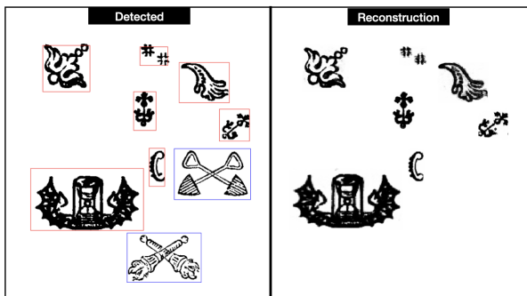
Fig. 5: DAE reconstructions with P = 0.2 (right) from input image (left).
