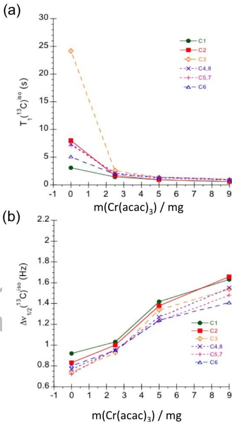
Figure 8. Variation of (a) T_1(^{13}\text{C})^{\text{iso}} and (b) \Delta\nu_{1/2}(^{13}\text{C})^{\text{iso}} of 2 (~100 mg) in chloroform (600 mg) versus the amount of \text{Cr}(\text{acac})_3 added (0.0, 2.5, 5.0 and 9.0 mg). Note the strong decrease in T_1(^{13}\text{C})^{\text{iso}} in the presence of \text{Cr}(\text{acac})_3 , especially for the C-3 carbon site.
