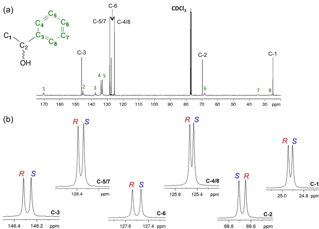
Figure 4. (a) 176.09 MHz ^{13}\text{C}\{-^1\text{H}\} 1D NMR spectrum of ( \pm )- 2 ( AS-5 ) in the PBLG/ \text{CDCl}_3 chiral mesophase at 303 K ( T_{\text{exp}} = 124 min, 120 scans and 4 dummy scans, X4 decoupling scheme). An exponential filtering ( \text{LB} = 1 Hz) is applied. ^{13}\text{C} -peaks labelled with a green number (1 to 8) originate from PBLG polymer side chain (see also Figure SI-4 ). Compared to the analyte ^{13}\text{C} signals, they are both smaller and larger ( T_2^{\text{PBLG}} < T_2^{\text{Solute}} ). (b) Zoom on each ^{13}\text{C} site. Spectra data are listed in Table 1 . The R/S assignment was made by comparison with the ^{13}\text{C}\{-^1\text{H}\} spectra of ( R )- 2 and ( S )- 2 as well as the comparison with a scalemic mixture of 2 ( \text{ee}(\text{S}) = 40\% ( AS-2 )). Note the inversion of spectral positions for S and R isomers at the carbon site C-2 compared to other sites.
