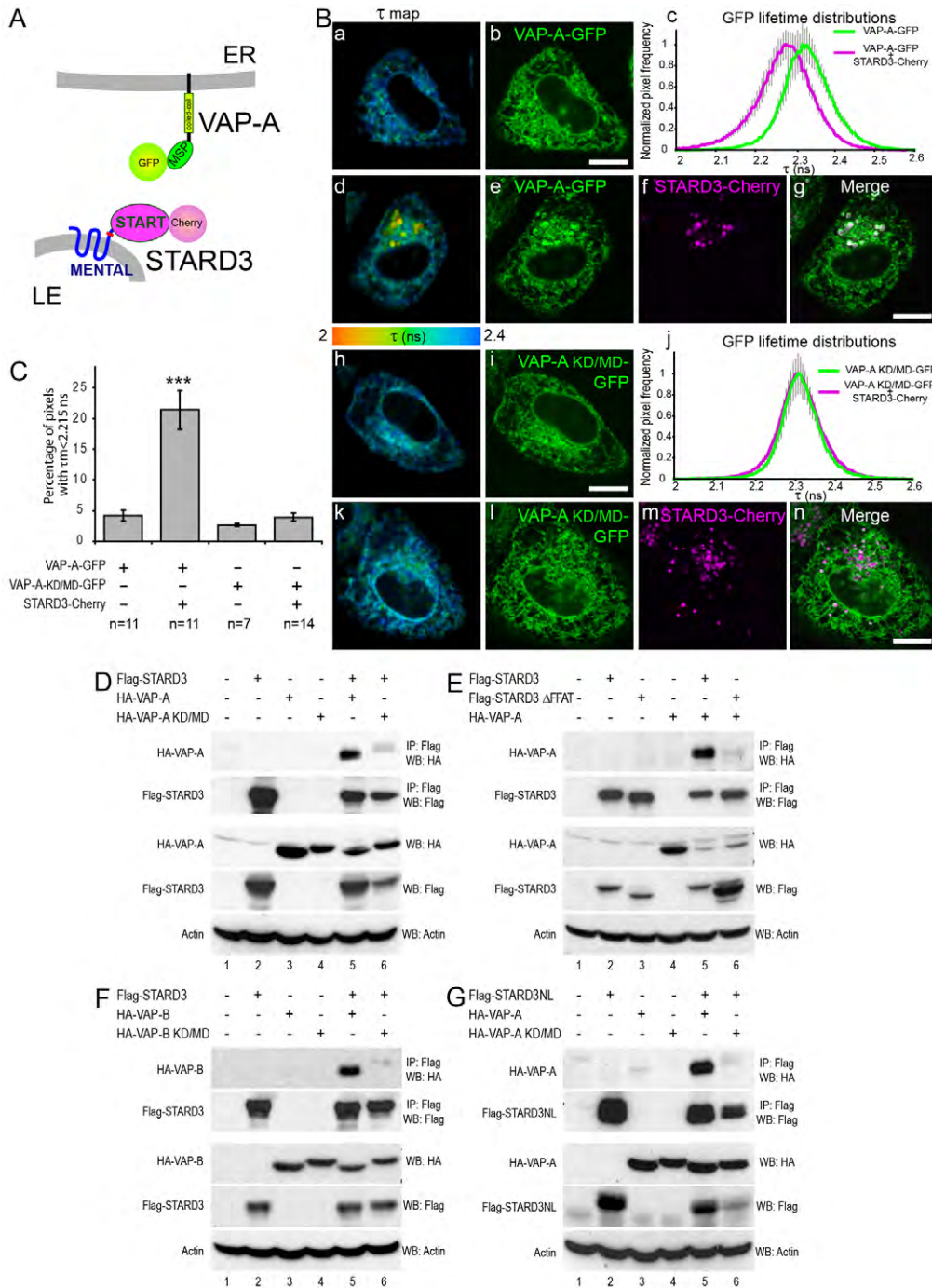
Fig. 3. STARD3 and STARD3NL interact with VAP proteins in a FFAT-motif-dependent manner.
