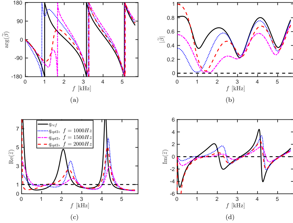
Figure 10: (a) Argument and (b) modulus of the reflection coefficient \tilde{\beta}(s) based on q_{ref} and q_{opt3} for the three analysed frequencies f . (c) Real and (d) imaginary part of the impedance \tilde{z}(s) . \tilde{z} = (1 + \tilde{\beta}) / (1 - \tilde{\beta}) .
