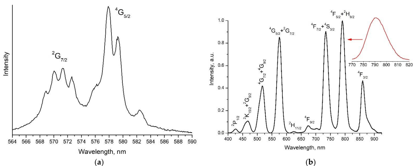
Figure 4. Fluorescence excitation spectrum of the 0.1 at% \text{Nd}^{3+} : \text{LaF}_3 type I NPs sample detected at 862.8 nm when scanning the laser within the {}^4\text{I}_{9/2} \rightarrow {}^4\text{G}_{5/2} + {}^2\text{G}_{7/2} transition wavelengths, normalized to the laser energy (a) and detected at 1064 nm in the range of 400–925 nm (b).
