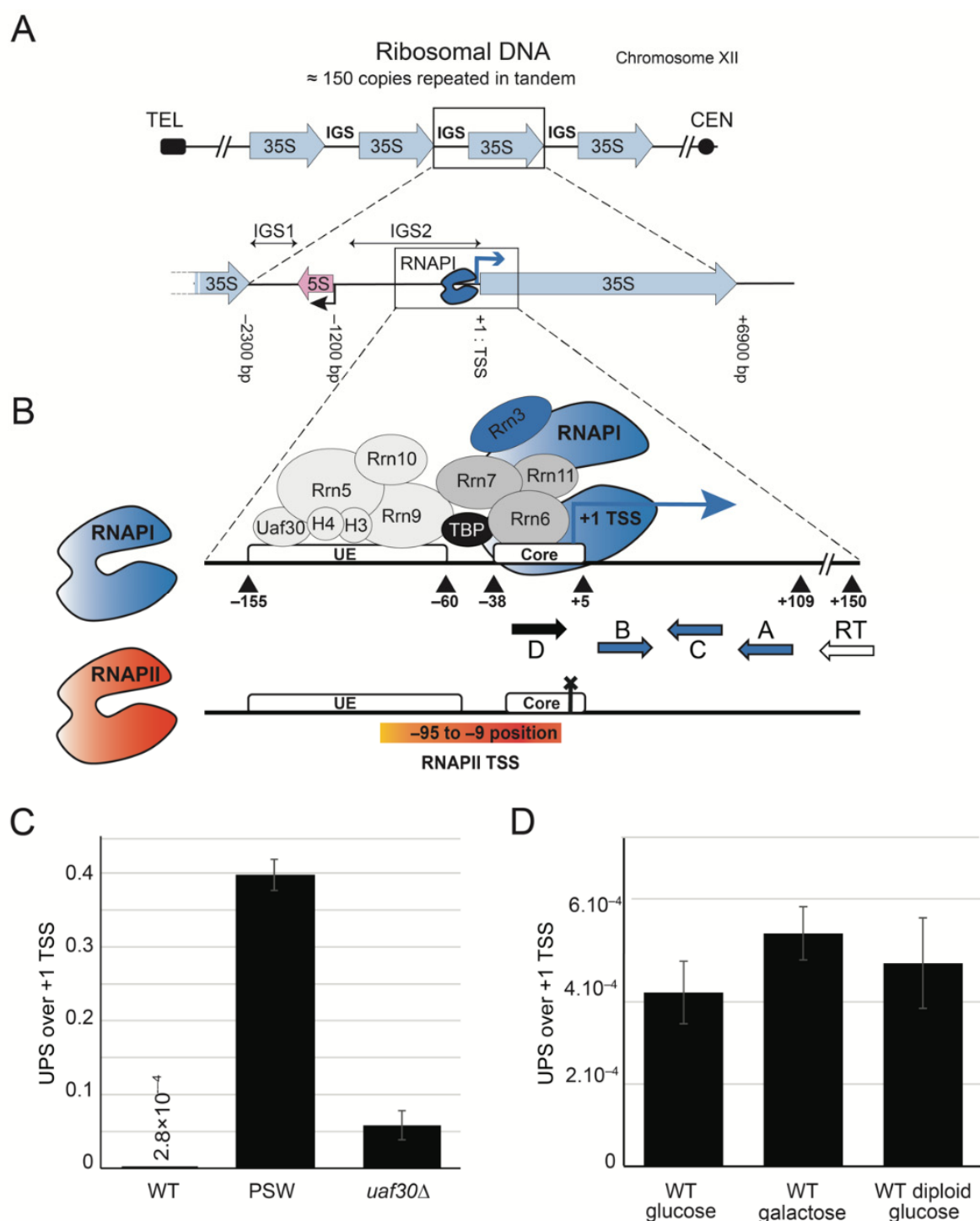
Figure 1. UPS lncRNAs are transcribed from the IGS2 region in rDNA. (A) Schematic representation of the rDNA locus in yeast Saccharomyces cerevisiae . The budding yeast contains a single rDNA cluster organized as a linear array of 100–150 rDNA repeats on chromosome XII. Each repeat, of 9.1-kb, produces a 35S precursor rRNA (35S gene is the blue arrow, sequence coordinates are relative to +1 TSS). IGS (intergenic sequence) is separated by the 5S gene (transcribed by RNAPIII, red arrow) into IGS1 and IGS2. (B) Details of the 35S promoter region composed of UE (Upstream Element) and core promoter. UE is occupied by the UAF complex (Uaf30, Rrn5, Rrn9, Rrn10, H3, and H4 subunits represented as light grey
