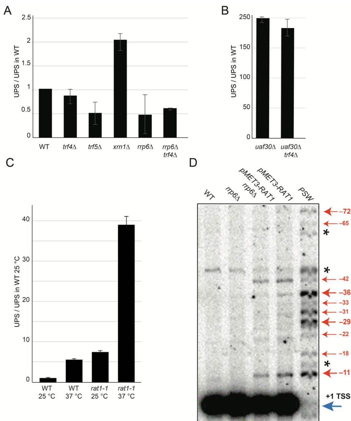
Figure 2. UPS are unstable lncRNAs degraded by Xrn1 and Rat1 5'-3' exoribonucleases. (A) UPS accumulate in xrn1Δ but not in exosomes ( rrp6Δ ) or in the TRAMP complex ( trf4Δ , trf5Δ ) mutants. Yeast cells were exponentially grown in YPD medium at 30 °C overnight. Quantification of UPS in RNA decay mutants using qPCR and primers are described in Figure 1B. Quantities of UPS in mutants are represented as a ratio to UPS quantities in wild type. Error bars correspond to the standard deviation of two or three independent cultures. (B) UPS accumulation in uaf30Δ and uaf30Δ trf4Δ mutants. UPS were quantified as described in (A). (C) UPS accumulate in rat1-1 mutated strain. WT and rat1-1 strains (BY4741) were grown overnight at 25 °C to early exponential phase and then shifted to 37 °C for 6 h. Quantification of UPS in RNA decay mutants using qPCR. Quantities of UPS in mutants are represented as a ratio to UPS quantities in wild type at 25 °C. Error bars correspond to standard deviation of two independent cultures. (D) Visualization of UPS in Rat1-depleted cells. Cells were cultivated in YPD medium than switched to YPD+ 6 mM methionine for 12 h. Primer extension reaction with radiolabeled RT primer (Figure 1B) was resolved in 10% denaturing acrylamide gel. UPS are marked by red arrows and +1 TSS is marked by the blue one (please note the saturated exposure of +1 TSS signal). Star (*) represents non-specific RT product.
