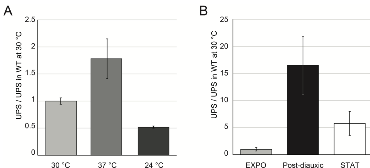
Figure 4. UPS transcripts accumulated in various growth conditions. (A) High temperature increased UPS level. Total RNA was extracted from wild-type cells cultivated overnight to exponential phase in YPD at indicated temperatures. UPS level was quantified as in Figure 1C. Error bars correspond to the standard deviation of three independent cultures. (B) UPS accumulated in post-diauxic and stationary (STAT) wild-type cells. Cells were grown in YPD at 30 °C overnight to the exponential phase (EXPO) and then left for either an additional 24 h or 11 days. RNA extraction and experimentation was performed as in Figure 1C, data were normalized by scR1 RNA reverse transcribed with specific primer ( scR1 -R), and quantified with an scR1 F/R couple. scR1 -normalized values were represented as a ratio of WT exponential values. Error bars correspond to the standard deviation of three independent cultures.
