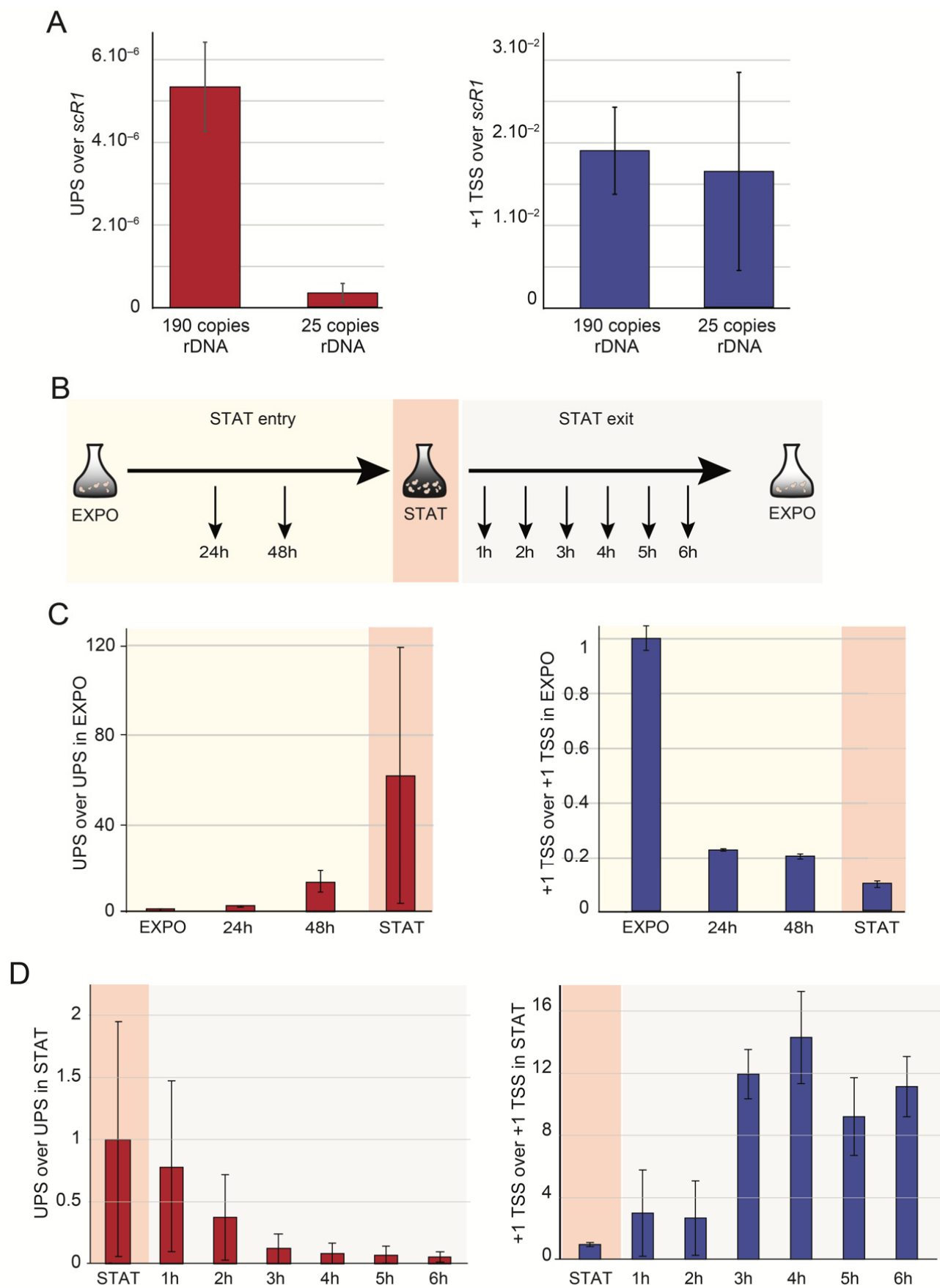
Figure 5. UPS are produced from closed rDNA copies, accumulated in quiescent cells, and anti-correlated with +1 TSS rRNA. (A) UPS levels were higher in 190-copy rDNA strains when compared to those with 25 rDNA copies. Strains bearing
