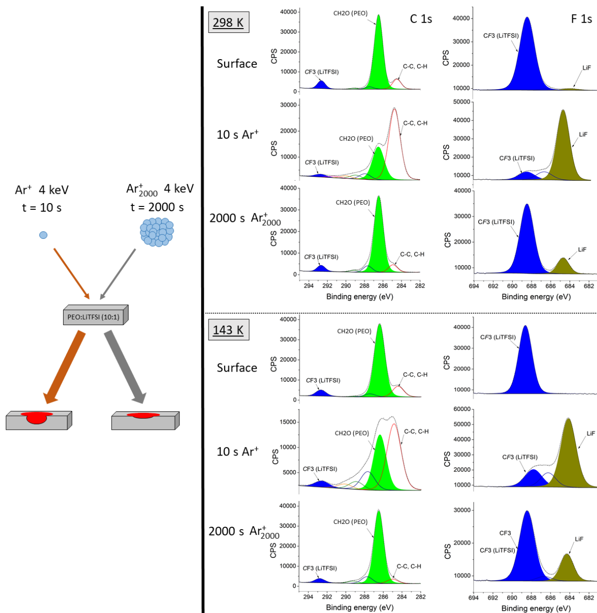
Figure 9. Depth profiling study on a PEO:LiTFSI (10:1) film using Ar + at 4 keV or Ar 2000 + at 4 keV (2 eV per Ar atom) as sputtering beam. The experimental data is represented by dots and the fitting line results from convolution of the proposed components.
