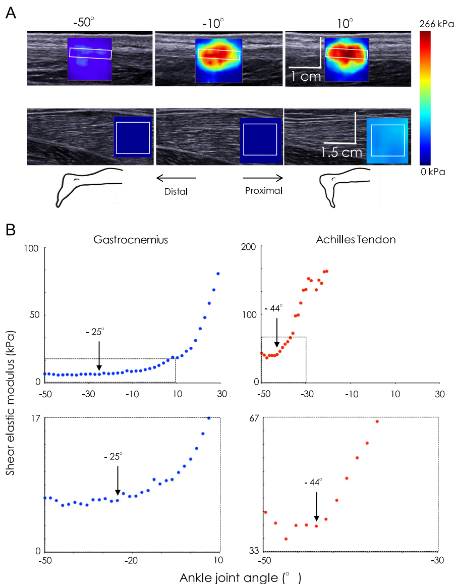
Fig. 1. Typical example of change in muscle and tendon shear elastic modulus during passive stretching. A—Maps of shear elastic modulus obtained at -50^\circ , -10^\circ and 10^\circ of ankle joint angle ( 0^\circ foot perpendicular to the leg) at 90^\circ of knee flexion. The scale is depicted at the right of the figure. The region of interest used to calculate the mean shear elastic modulus is drawn in white. B—Relationship between shear elastic modulus and ankle joint for both gastrocnemius medialis and Achilles tendon (knee angle =0^\circ ). The bottom panels correspond to a zoom of the region of interest defined as the rectangle on the top panels. These zoomed traces were used to detect the ankle angle corresponding to the slack length (indicated by an arrow).
