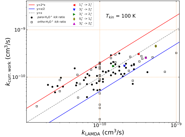
Figure 7. State-to-state ratios of our recent thermal rate coefficients and the corresponding data listed in the LAMDA data base (Schöier et al. 2005). The collisional data both for o - \text{H}_3\text{O}^+ and p - \text{H}_3\text{O}^+ are considered at 100 K kinetic temperature.
