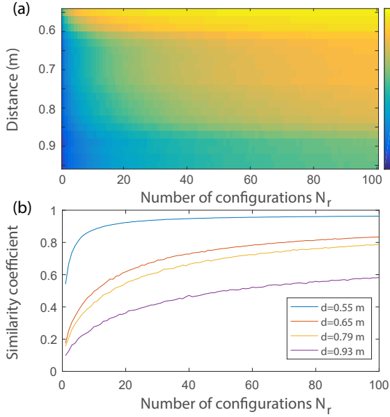
FIG. 5. (a) Colormap of the similarity coefficient S(N_r, d) shown as a function of the number of configurations N_r over which the averaging is performed and the distance d between the receiving antennas.
