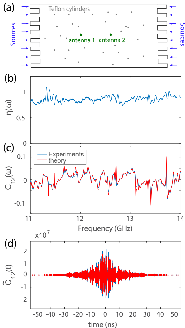
FIG. 2. (a) Schematic drawing of the 2D experimental setup used to reconstruct the impulse response between two wire antennas located near the middle of the cavity. The spacing between the wire antennas is d = 0.06 m. (b) Variations of \eta(\omega) with frequency. (c) Real part of the cross-correlation as a function of frequency, C_{12}(\omega) (blue), and corresponding results from Eqs. (3) and (5) (red). (d) Time domain representation of the results displayed in (c).
