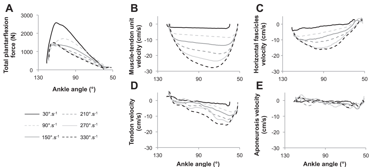
Fig. 2. Patterns of shortening velocity of musculotendinous elements measured during plantar flexions at different movement speed for the gastrocnemius medialis. A: total plantar flexion force. B: MTU velocity. C: horizontal fascicles velocity. D: tendon velocity. E: aponeurosis velocity. Error bars were omitted for clarity.
