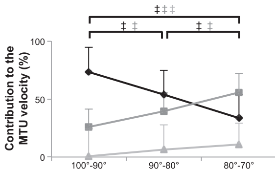
Fig. 4. Relative contributions of elements (fascicles: solid diamonds; tendon: medium-shaded squares; aponeurosis: light-shaded triangles) to global MTU velocity on the different angular range (100–90°, 90–80°, 80–70°). ‡Significant difference with the other angular ranges of the element considered ( P < 0.001 ).
