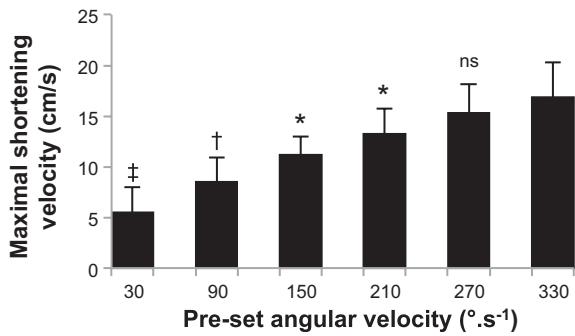
Fig. 7. Maximal shortening velocity of fascicles for each preset angular velocity. Significant differences between the considered velocity and the higher velocity: * P < 0.05 , † P < 0.01 , and ‡ P < 0.001 . ns, Nonsignificant.
