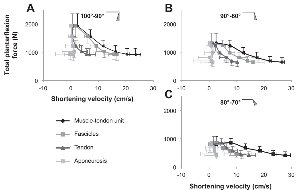
Fig. 6. Force-velocity relationships of the MTU, fascicles, tendon, and aponeurosis on the three considered angular range of motion [100–90° (A), 90–80° (B), 80–70° (C), with 90° corresponding to the foot being perpendicular to the leg and a decreased angle for the plantar flexion].
