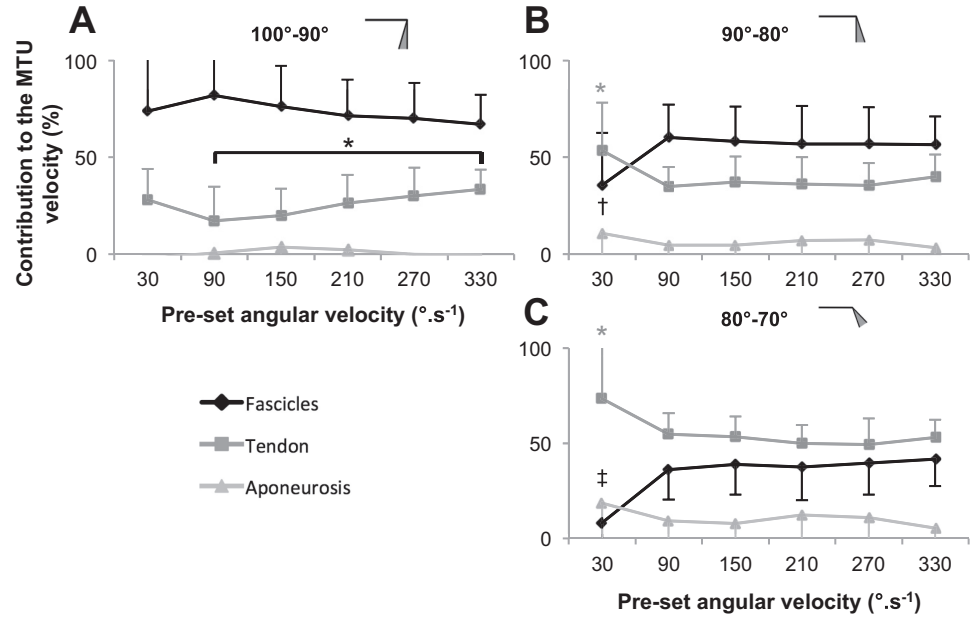
Fig. 5. Relative contributions of elements (fascicles: solid diamonds; tendon: medium-shaded squares; aponeurosis: light-shaded triangles) to the global MTU velocity in isokinetic trials, on three angular ranges [100–90° (A), 90–80° (B), 80–70° (C), with 90° corresponding to the foot being perpendicular to the leg and a decreased angle for the plantar flexion]. Significant difference between the considered angular velocity and the fastest angular velocity: * P < 0.05 , † P < 0.01 , and ‡ P < 0.001 . All of the other contributions were not significantly ( P > 0.05 ) different from the contribution of the same element at the fastest velocity.
