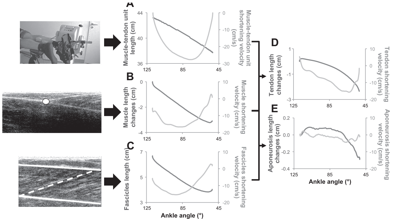
Fig. 1. Individual examples of lengths and velocities measurements at an isokinetic velocity of 330°/s. A : the isokinetic dynamometer was used to measure ankle angle and angular velocity, and the muscle-tendon unit (MTU) length was estimated using the model of Grieve et al. (24). B : the ultrasound scanner was used to manually track the myotendinous junction (white point), to estimate the change in length of the muscle. C : the ultrasound scanner was also used to measure the fascicle length change (white dotted line) and the aponeurosis behavior (white line) using the automatic tracking procedure of Cronin et al. (12). D : the tendon length change was estimated as the MTU length change minus the muscle length change. E : the aponeurosis length change was estimated as the muscle length change minus the horizontal fascicle length change. The temporal derivative of the changes in length was calculated to obtain the shortening velocity of each element.
