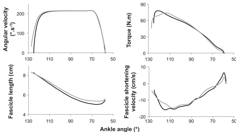
Fig. 8. Individual example of angular velocity, torque, and length and shortening velocity of fascicles at an isokinetic velocity of 210°/s between two start conditions: with an active dorsiflexion (solid line), and a dorsiflexion performed by the experimenter and with a started static position (shaded line).
