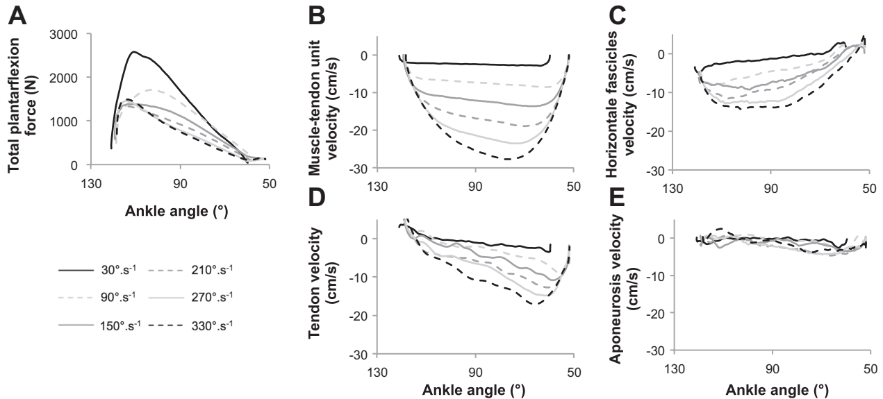
Fig. 3. Patterns of shortening velocity of musculotendinous elements measured during plantar flexions at different movement speed for the gastrocnemius lateralis. A: total plantar flexion force. B: MTU velocity. C: horizontal fascicles velocity. D: tendon velocity. E: aponeurosis velocity. Error bars were omitted for clarity.
