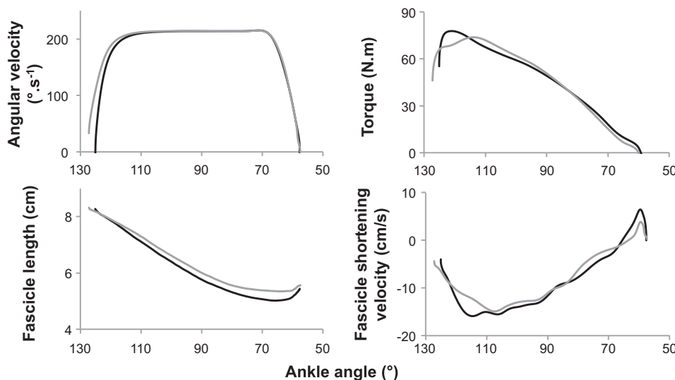
Fig. 8. Individual example of angular velocity, torque, and length and shortening velocity of fascicles at an isokinetic velocity of 210°/s between two start conditions: with an active dorsiflexion (solid line), and a dorsiflexion performed by the experimenter and with a started static position (shaded line).
