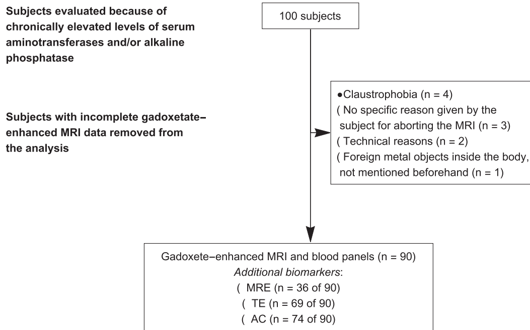
Figure 3. Data availability.
