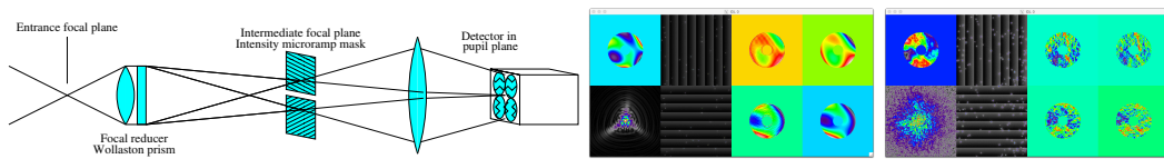
Fig. 1. Left: schematic concept of the VFWFS, with a mask in the focal plane, introducing an optical differentiation operation, and measurement in the pupil plane. Middle & Right: example of reconstructed wavefront derivatives for low order aberrations and a turbulent wavefront respectively.
