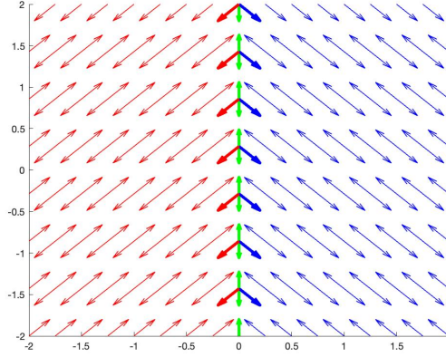
FIG. 2.3. Dynamics of Example 6.
