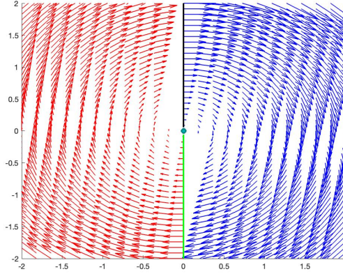
FIG. 2.4. The dynamics: In red the dynamics F_1(\cdot) and in blue the dynamics F_2(\cdot) .
