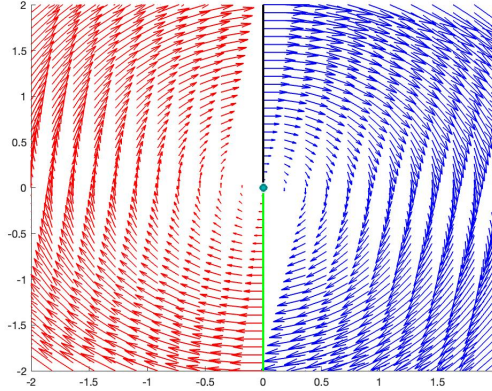
FIG. 2.4. The dynamics: In red the dynamics F_1(\cdot) and in blue the dynamics F_2(\cdot) .
