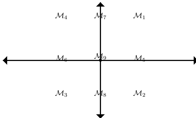
FIG. 2.2. Example of a stratification of \mathbb{R}^2 .
