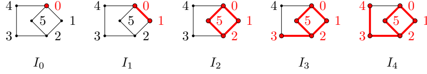
FIGURE 2. Constructing a clique in \text{Cayley}(\Lambda, \text{Vor}(\Lambda)) from the Delaunay graph D(\Lambda, \{v_0, \dots, v_n\}) .
