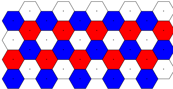
FIGURE 1. Optimal coloring of the hexagonal lattice, \chi(A_2) = 3 .
