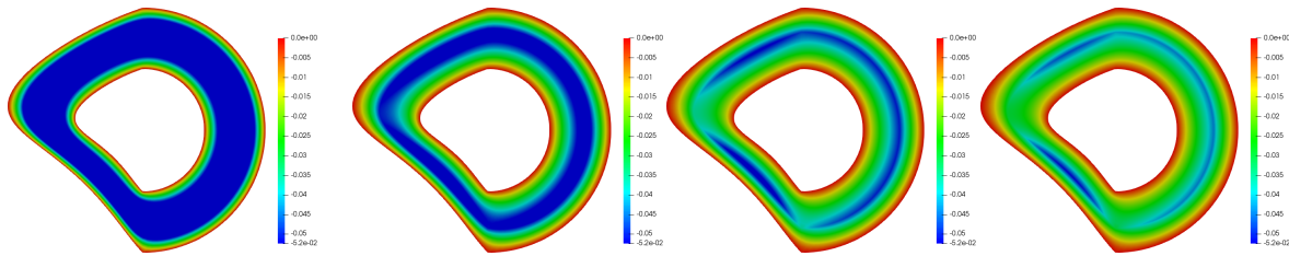
Fig. 11: Propagation of the \varphi_r(t) field at t_1 = 0, t_2 = 2.43, t_3 = 3.47 and t_4 = 4 .
