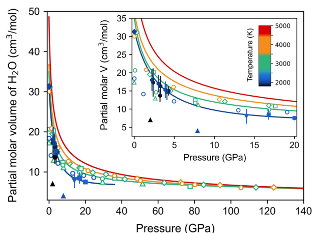
Figure 3. Partial molar volumes of \text{H}_2\text{O} in magmatic melts. Curves are the results of our simulations of pyrolite + 4\text{H}_2\text{O} (2.2 wt% \text{H}_2\text{O} ) at 2000 K (blue), 3000 K (green), 4000 K (orange) and 5000 K (red). Experimental data are shown as filled symbols: albite melt with 1.9–6.1 wt% \text{H}_2\text{O} at 2000 K (diamond; Ochs & Lange, 1997), pyrolite melt with 5 wt% \text{H}_2\text{O} at 2170 K (downward-pointing triangles; Matsukage et al., 2005), basalt melt with 8 wt% \text{H}_2\text{O} at 2200 K (squares; Sakamaki et al., 2006), komatiite-fayalite mixture with 2–5 wt% \text{H}_2\text{O} at 1773 and 2073 K (upward-pointing triangles; Agee, 2008), and peridotite melt with 5 wt% \text{H}_2\text{O} at 1773–2073 K (circles; Sakamaki et al., 2009). Data from ab initio molecular dynamics simulations are shown as open symbols: silica melt with 8.25 wt% \text{H}_2\text{O} at 3000 K (open triangles; Bajgain et al., 2015; Karki & Stixrude, 2010), enstatite melt with 4.5 wt% \text{H}_2\text{O} at 3000–4000 K (open diamonds; Karki et al., 2020), enstatite melt with 10 wt% \text{H}_2\text{O} at 3000 K (open squares; Mookherjee et al., 2008), and basalt melt with 5 wt% \text{H}_2\text{O} at 2200–4000 K (Bajgain et al., 2015). Inset shows a magnification of the 0–20 GPa region.
