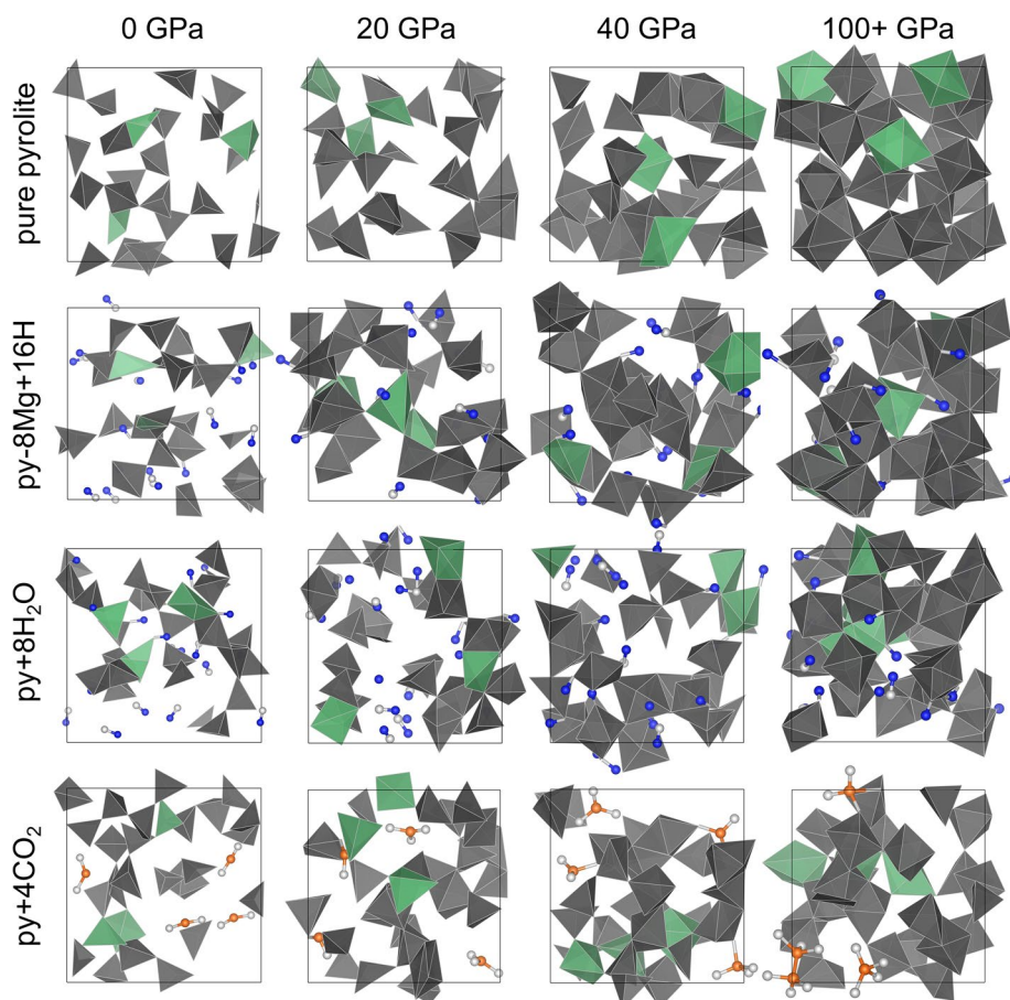
Figure 5. The evolution of the silica-alumina network in volatile-free and volatile-bearing pyrolite melts as a function of pressure at 4000 K. Mg, Fe, Ca, and Na polyhedra are omitted to show the silica-alumina polymerization network. Only the silica polyhedra (gray), alumina polyhedra (green), hydrogen atoms (blue), carbon atoms (orange), and (C,H)-bonded oxygen atoms (white) are shown. Simulations are conducted at constant density. The exact pressure of each simulation is 0, 15, 48, and 148 GPa for pure pyrolite (first row); 0, 24, 43 and, 132 GPa for py-8Mg+16H (second row); 0, 22, 38, and 113 GPa for py+8H 2 O (third row); and 0, 20, 36, and 108 GPa for py+4CO 2 (fourth row). It should be noted that each cell is an example of only one step out of tens of thousands of time steps from the simulations.
