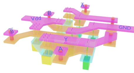
Fig. 13. 3D representation of XOR gate.
