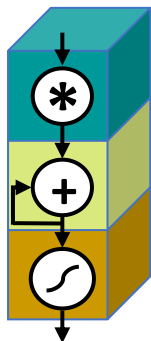
Fig. 20. Versatile VNWFEF-logic based 3D neural network compute cube ( N^2C^2 ).
