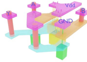
Fig. 11. 3D representation of NAND gate.
