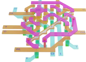
Fig. 16. Non-volatile 1-bit full adder.
