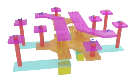
Fig. 19. Non-volatile circuit tile based on ambipolar reconfigurable FETs.
