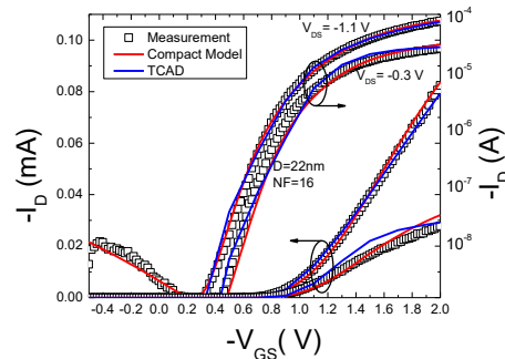
Fig. 2. Model calibration for JL VNW-FETs.
