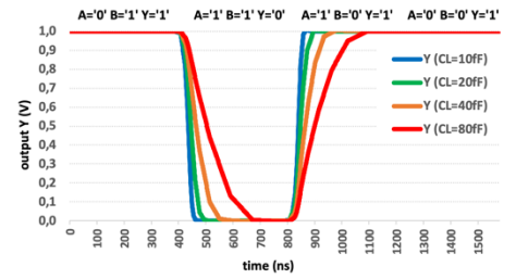
Fig. 14. Transient simulation of the NAND gate.
