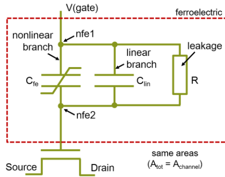
Fig. 5. Schematic of the Preisach-based Verilog-A FeCap model as gate extension for the VJLNW-FETs.
