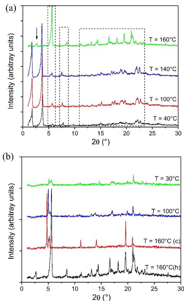
Fig. 3. X-ray diffraction patterns of I-4 recorded on heating (a) and cooling (b) at different temperatures.
