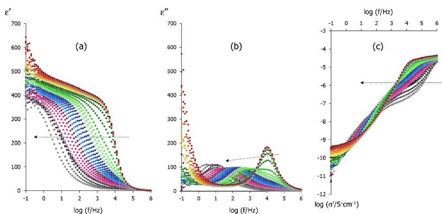
Fig. 10. Dielectric and conductivity response of II-3 as a function of the frequency, measured at different temperatures on cooling from T = 160\ \text{°C} to room temperature ( T = 32\ \text{°C} ): (a) dielectric elastic constant, \epsilon' ; (b) loss modulus, \epsilon'' ; (c) real component of the complex conductivity, \sigma' . Arrows indicate direction on cooling.
