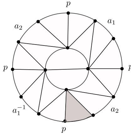
FIGURE 7. An associated disk P to the word w = a_1 a_2 a_1^{-1} a_2
