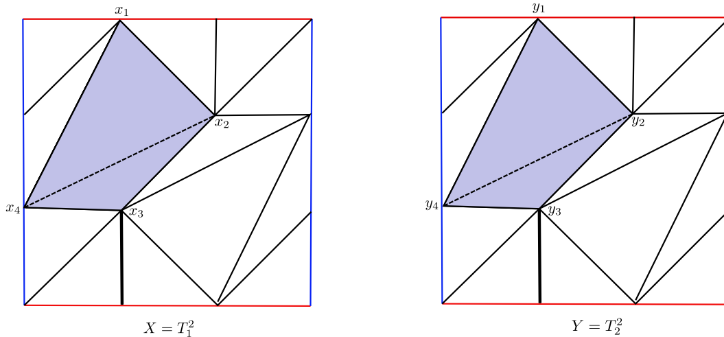
FIGURE 1. Minimal triangulation of a torus T^2
