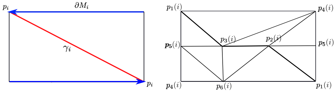
FIGURE 5. The triangulation of the Möbius band.
