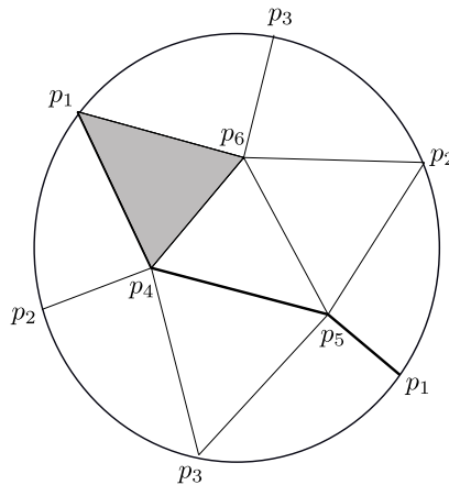
FIGURE 2. Minimal Triangulation of \mathbb{R}P^2
