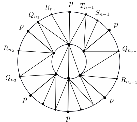
FIGURE 6. Triangulation of disk D_1^2 for s = 6
