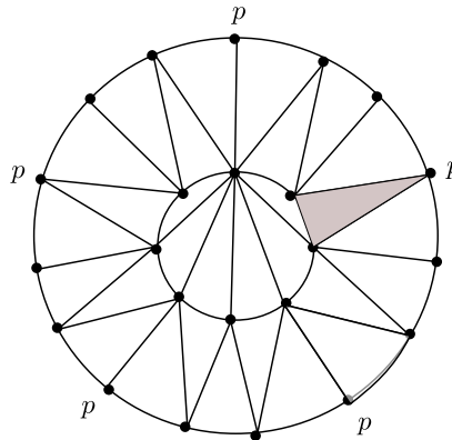
FIGURE 4. Triangulation of the disk P_l for odd l ( l = 5 ).
