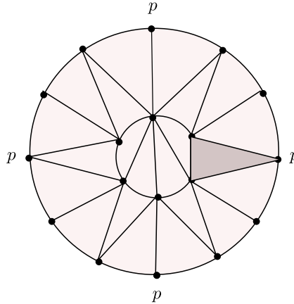
FIGURE 3. Triangulation of the disk P_l for even l ( l = 4 ).
