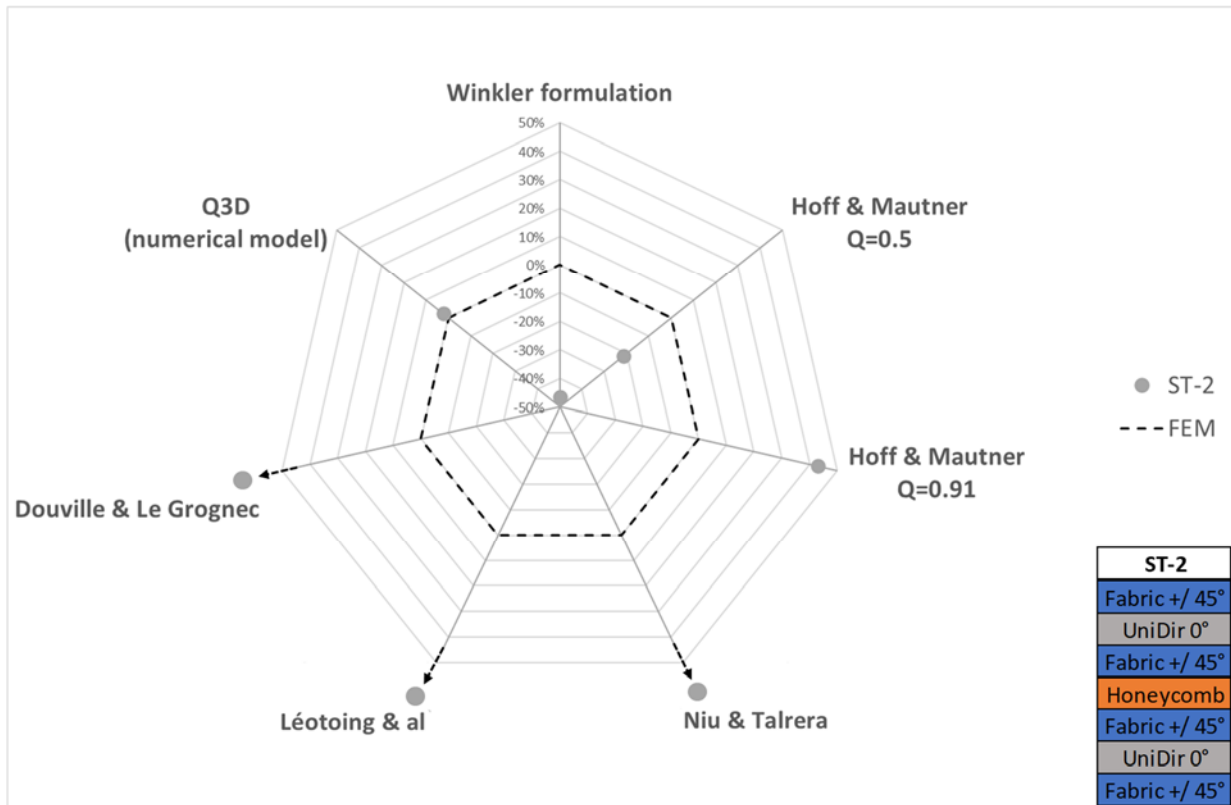
Figure 9: Radar type comparison graph for ST-2 sandwich stacking: Symmetric balanced orthotropic skin with honeycomb core
