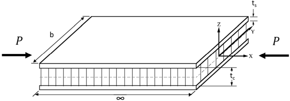
Figure 5: Geometry of analytical models
