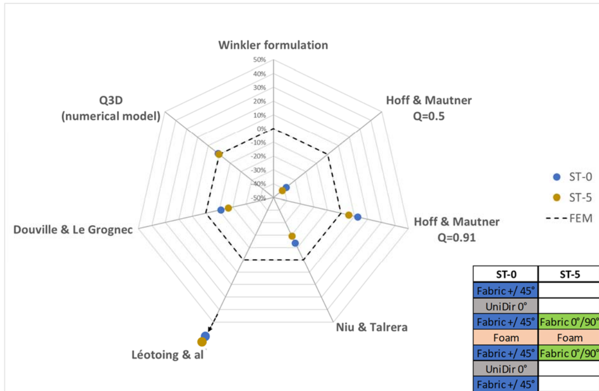
Figure 12: Radar type comparison graph for ST-0 and ST-5 with a single ply
