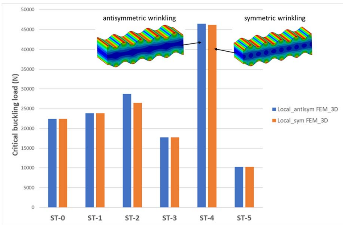
Figure 7: 3D FEM critical local buckling load for antisymmetric and symmetric modes
