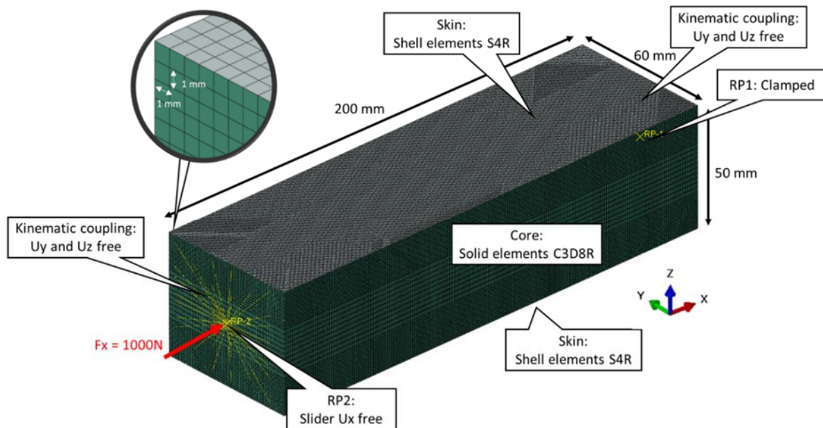
Figure 4: 3D FEM with its boundary conditions
