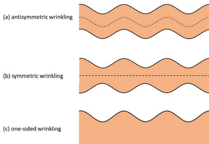
Figure 2: The different wrinkling modes.
