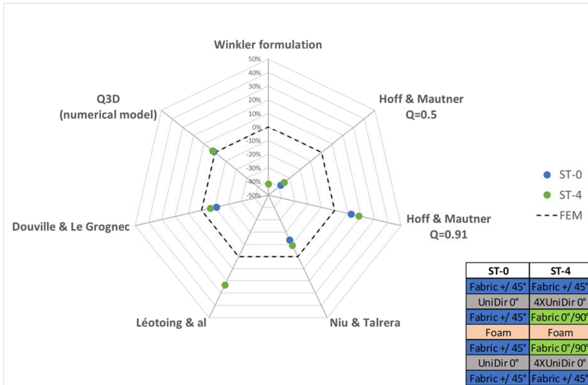
Figure 11: Radar type comparison graph for ST-0 and ST-4 with a large proportion of UniDirectional ply
