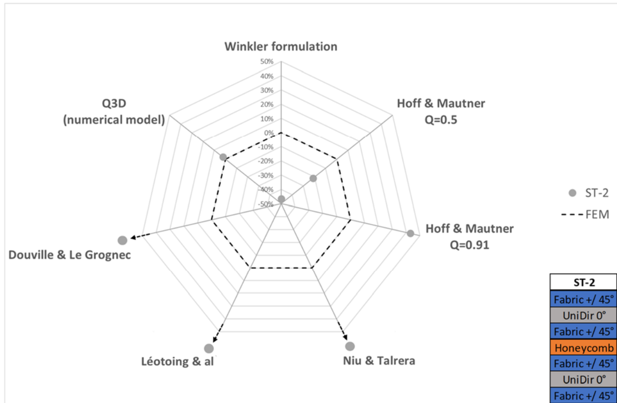
Figure 9: Radar type comparison graph for ST-2 sandwich stacking: Symmetric balanced orthotropic skin with honeycomb core
