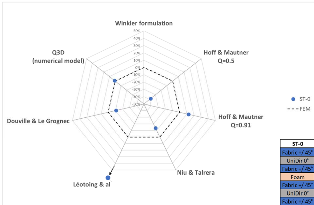
Figure 8: Radar type comparison graph for ST-0 sandwich stacking: symmetric balanced orthotropic skin with foam core.
