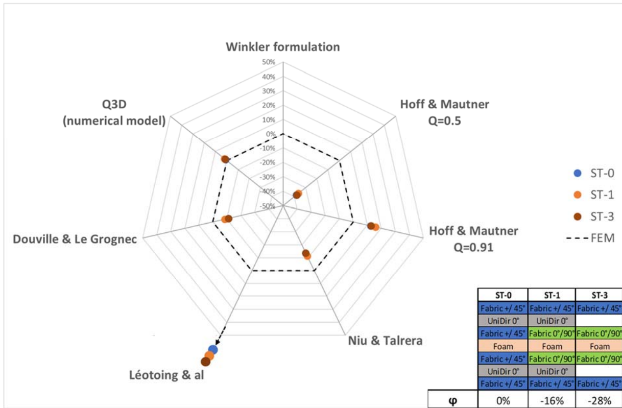
Figure 10: Radar type comparison graph for symmetric skins (ST-0) and asymmetric skin (ST-1; ST-3)
