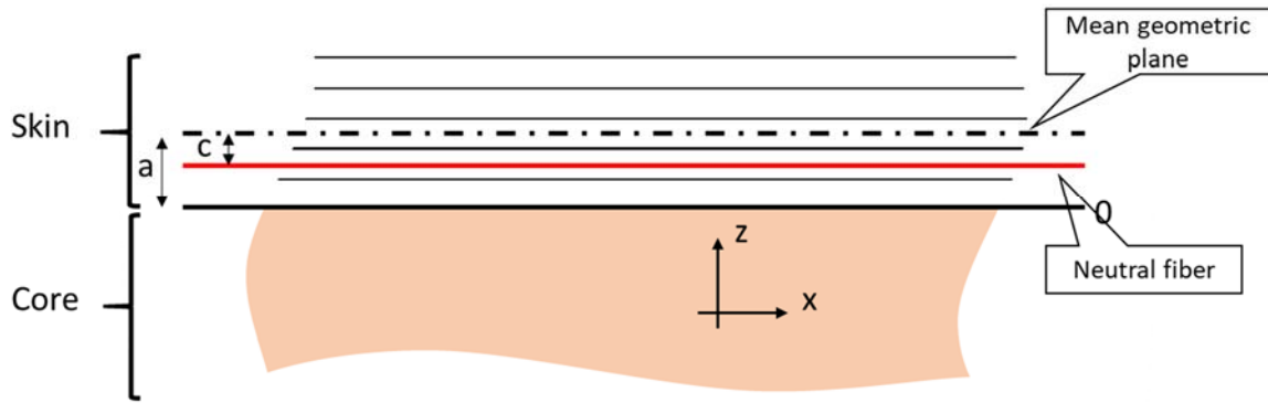
Figure 6: Definition of the asymmetry parameter \varphi
