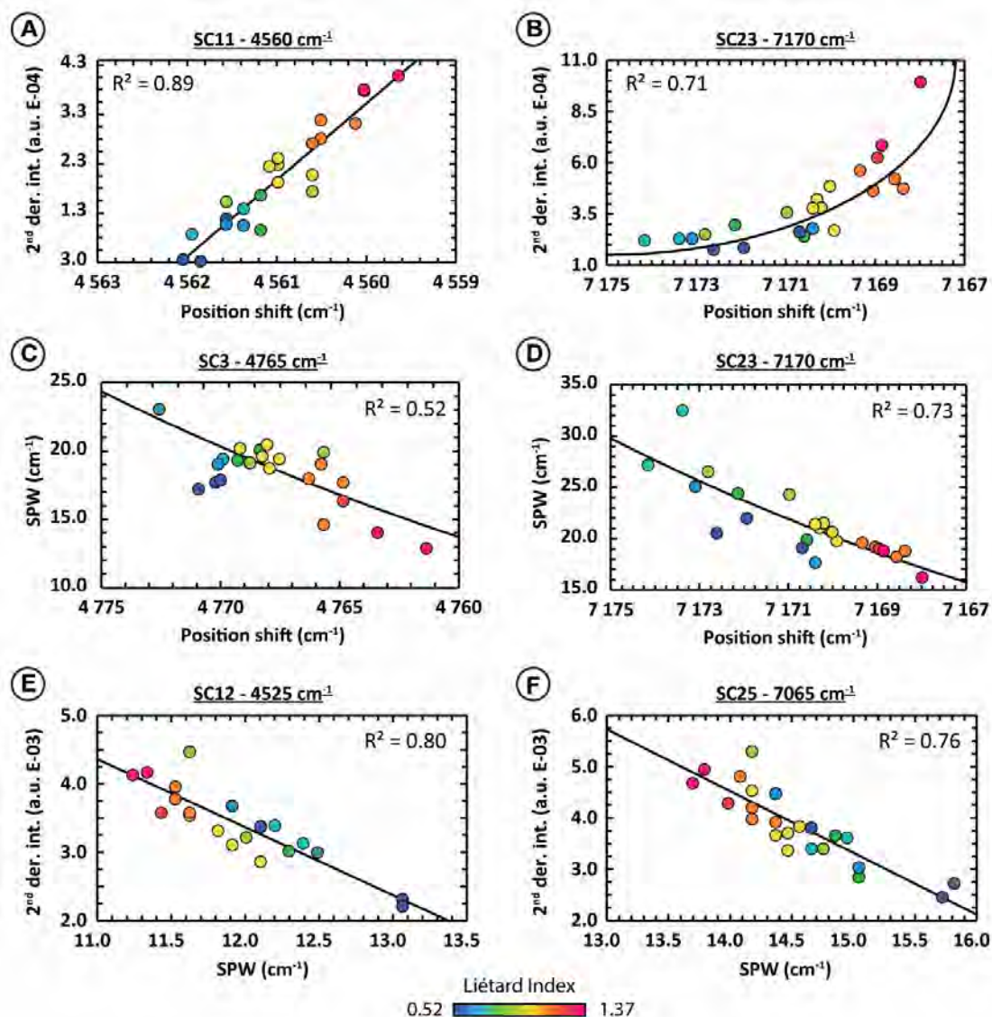
Figure 8 - Relationship between the different spectral parameters. (A) 2 nd derivative local maxima intensities as function of the shifts in position of the 4560 cm -1 SC11. (B) 2 nd derivative local maxima intensities as function of the shifts in position of the 7170 cm -1 SC23. (C) SPW values as function of the shifts in position of the 4765 cm -1 SC3. (D) SPW values as function of the shifts in position of the 7170 cm -1 SC23. (E) 2 nd derivative local maxima intensities as function of the SPW values of the 4525 cm -1 SC12. (F) 2 nd derivative local maxima intensities as function of the SPW values of the 7065 cm -1 SC25. Data points are colorized according to the Liétard Index LI values that increase with the crystalline order (key at bottom of spectral plot). Experimental spectral resolution is about 2.0 cm -1 , numerically resampled to 0.1 cm -1 using the cubic spline interpolation method.
