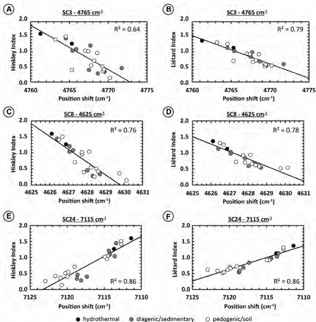
Figure 9 - Relationship between the shifts in position of different SCs and XRD indices. (A) Shifts in position of the 4765 cm -1 SC3 as function of the Hinkley Index. (B) Shifts in position of the 4765 cm -1 SC3 as function of the Liétard Index. (C) Shifts in position of the 4625 cm -1 SC8 as function of the Hinkley Index. (D) Shifts in position of the 4625 cm -1 SC8 as function of the Liétard Index. (E) Shifts in position of the 7115 cm -1 SC24 as function of the Hinkley Index. (F) Shifts in position of the 7115 cm -1 SC24 as function of the Liétard Index. Experimental spectral resolution is about 2 cm -1 , numerically resampled to 0.1 cm -1 using the cubic spline interpolation method.
