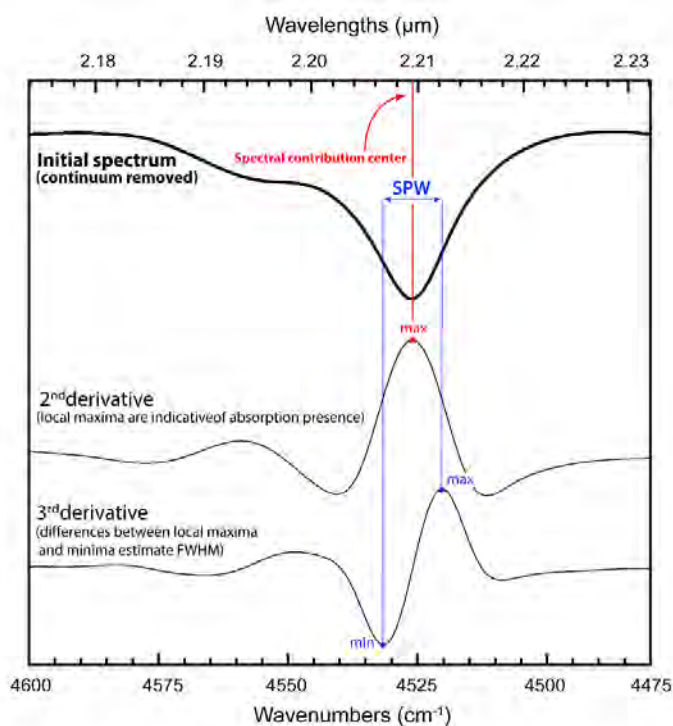
Figure 4 - Illustration of the calculations of the spectral contribution center and its SPW in a kaolinite spectrum from the second and third derivatives respectively. The chosen example is a zoom of the inner-OH vibration at 4525\text{ cm}^{-1} of the spectrum of the well-ordered kaolinite sample DCV from Decazeville, France.
