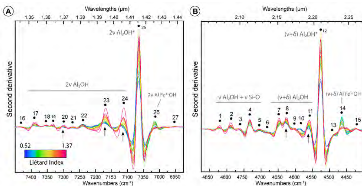
Figure 7 - Second derivative spectra of the two absorption bands at 7000\text{ cm}^{-1} (A) and 4500\text{ cm}^{-1} (B) of terrestrial kaolinites. Spectra are colorized according to the Liétard Index LI values that increase with the crystalline order (key at bottom of spectral plot). Vibrations modes: \nu = stretching; \delta = bending. The asterisk indicates absorptions associated to the inner-hydroxyl vibrations. Black dots indicate spectral contributions SC that were found through second derivative analysis. Black arrows point to remarkable “rainbow fan” distribution features caused by second derivative intensity regularly increasing with Liétard Index. Experimental spectral resolution is about 2.0\text{ cm}^{-1} , numerically increased resampled to 0.1\text{ cm}^{-1} using the cubic spline interpolation method.
