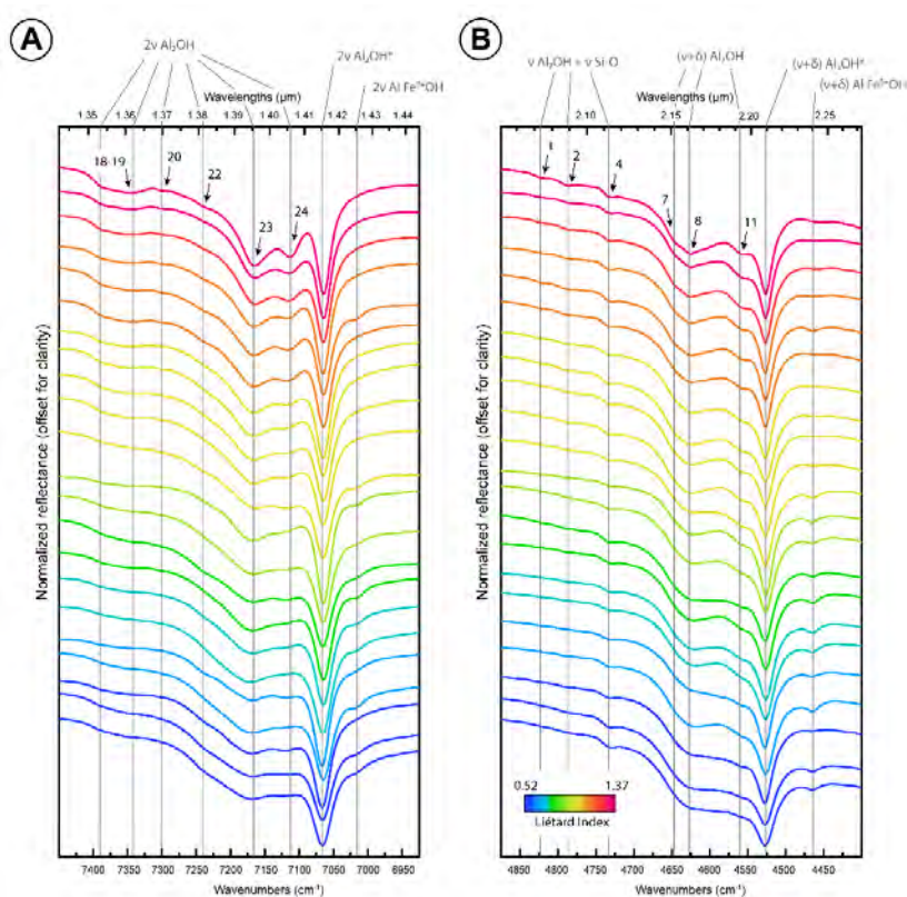
Figure 6 - Near-infrared reflectance spectra of the two absorption bands at 7000 cm -1 ( A ) and 4500 cm -1 ( B ) of terrestrial kaolinites. Spectra are colorized according to the Liétard Index LI values that increase with the crystalline order (key at bottom of spectral plot). Vibrations modes: ν = stretching; δ = bending. The asterisk indicates absorptions associated to the inner-hydroxyl vibrations. The black arrows point to absorptions that get more complex and/or intense as the crystallinity increases (numbers on top of black arrows indicate the spectral contributions SC identified with second derivatives; see Figure 7 and Table 2).
