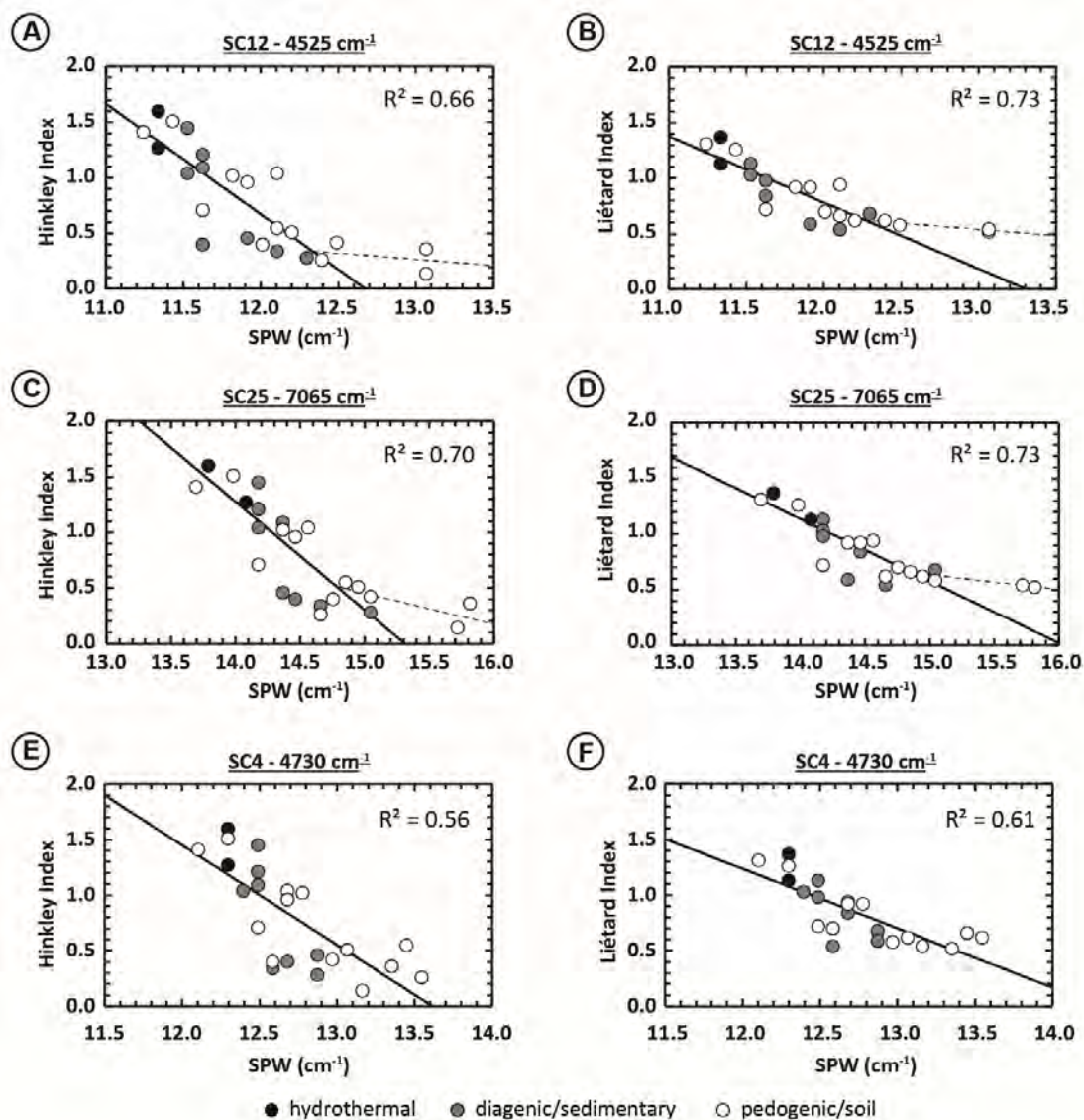
Figure 11 - Relationship between the SPW of different SCs and XRD indices. (A) SPW variation of the 4525 cm -1 SC12 as function of the Hinkley Index. (B) SPW variation of the 4525 cm -1 SC12 as function of the Liétard Index. (C) SPW variation of the 7065 cm -1 SC25 as function of the Hinkley Index. (D) SPW variation of the 7065 cm -1 SC25 as function of the Liétard Index. (E) SPW variation of the 4730 cm -1 SC4 as function of the Hinkley Index. (F) SPW variation of the 4730 cm -1 SC4 as function of the Liétard Index. Experimental spectral resolution is about 2 cm -1 , numerically resampled to 0.1 cm -1 using the cubic spline interpolation method. Note that correlation coefficients for SC12 and SC25 are calculated excluding the P2-150 and P1-300 samples (A,B,C and D figure parts). Dashed lines running through the P2-150 and P1-300 poorly-ordered samples were drawn to take into account the threshold effect explained in the subsection “Spectral significance of parameters variations” in the “Discussion” section.
