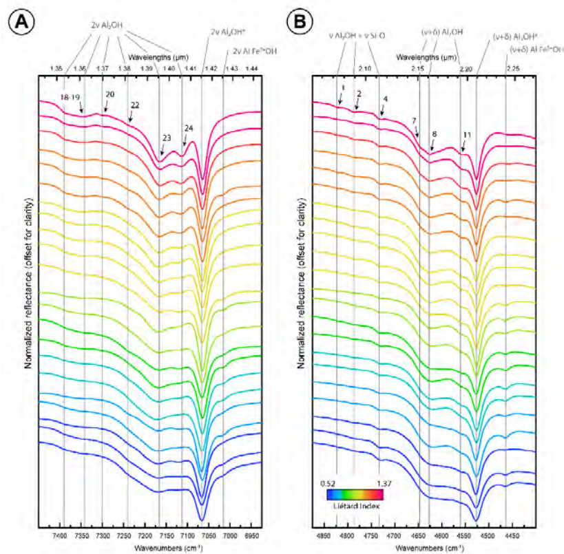
Figure 6 - Near-infrared reflectance spectra of the two absorption bands at 7000 cm -1 (A) and 4500 cm -1 (B) of terrestrial kaolinites. Spectra are colorized according to the Liétard Index LI values that increase with the crystalline order (key at bottom of spectral plot). Vibrations modes: ν = stretching; δ = bending. The asterisk indicates absorptions associated to the inner-hydroxyl vibrations. The black arrows point to absorptions that get more complex and/or intense as the crystallinity increases (numbers on top of black arrows indicate the spectral contributions SC identified with second derivatives; see Figure 7 and Table 2).
