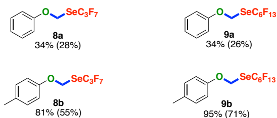
Scheme 3. Synthesis of R_F\text{SeCH}_2\text{O} -molecules. Yields determined by ^{19}\text{F} NMR with \text{PhOCF}_3 as internal standard; in parentheses, isolated yields.
