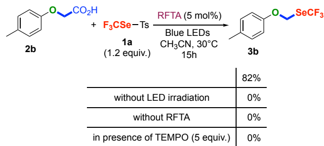
Scheme 5. Control reactions.
