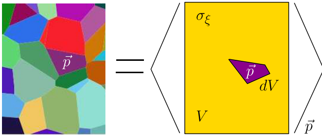
FIG. 4. Application of the effective medium theory to obtain the overall conductivity \sigma_\xi of the multigrained material with imperfect interfaces. The structure on the right is averaged over the properties \vec{p} = (\sigma_k \forall k = 1, \dots, d; R; r if \xi = LC or g if \xi = HC ) of the added grain.
