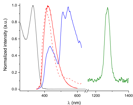
Figure 8. Normalized absorption (black), emission ( \lambda_{\text{exc}} = 325 nm) spectra for \text{GdL}^2 in dichloromethane at room temperature (red trace), 77K (dashed red) and after application of a 0.1 ms delay (blue). The green spectrum in the NIR is representative for the singlet oxygen luminescence.
