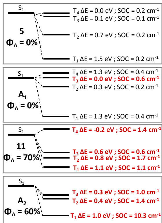
Figure 6. Computed Spin-orbit Coupling for the ( S_1 , T_1 ), ( S_1 , T_2 ), ( S_1 , T_2 ) and ( S_1 , T_4 ) states along with their energy differences and the experimental value of singlet oxygen generation efficiency. In red, SOCs larger than 0.5 \text{cm}^{-1} .
