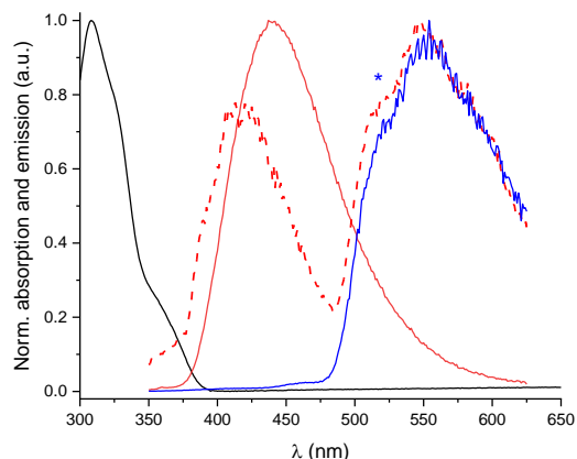
Figure 4. Normalized absorption (black) and emission (red) of A 2 in dichloromethane at room temperature, 77K emission
