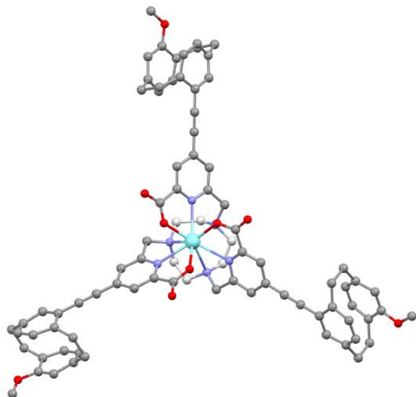
Figure 2. DFT optimized [YL^1] structure. Hydrogen atoms are omitted for clarity, C are represented in gray, O in red, N in blue and Y in cyan.
