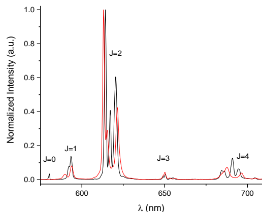
Figure 7. Normalized emission ( \lambda_{\text{exc}} = 325 \text{ nm} ) spectra of EuL 1 in dichloromethane at room temperature (red trace) and 77K (black trace). The nature of the {}^5\text{D}_0 \rightarrow {}^7\text{F}_j transitions are indicated.
