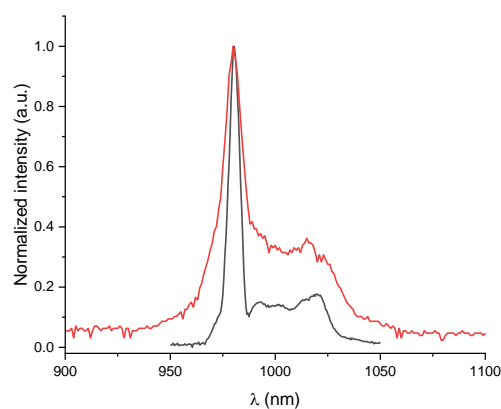
Figure 2. Normalized emission ( \lambda_{\text{exc}} = 325 nm) spectra for \text{YbL}^2 in MeOH-EtOH (1-4 vol) at room temperature (red trace) and 77K (black trace).
