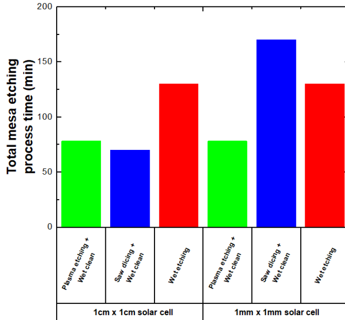
FIGURE 4. Mesa isolation process time required for each technique and for two different cell sizes.
