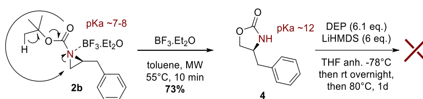
Scheme 2. Synthesis of the oxazolidine-2-one 4 from 2b using previously published procedure 34 and its lack of reactivity towards nucleophilic attack of diethylphosphite. The chelation model and the proposed mechanism for the ring expansion of N -Boc-aziridines into oxazolines catalyzed by azaphilic Lewis acids is well-known in the literature. 35,36
