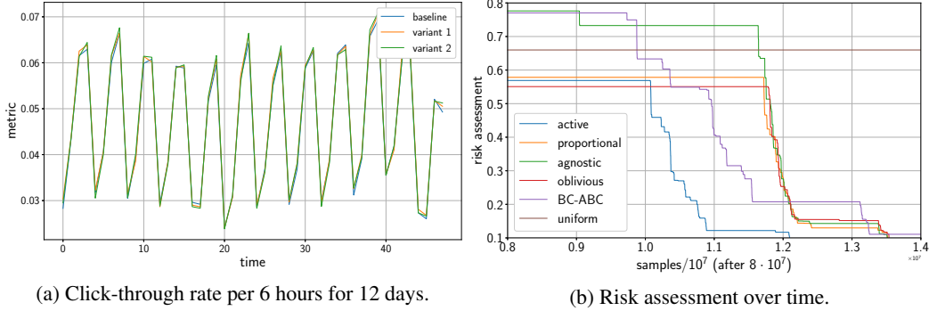
Figure 3: Real data and results.
