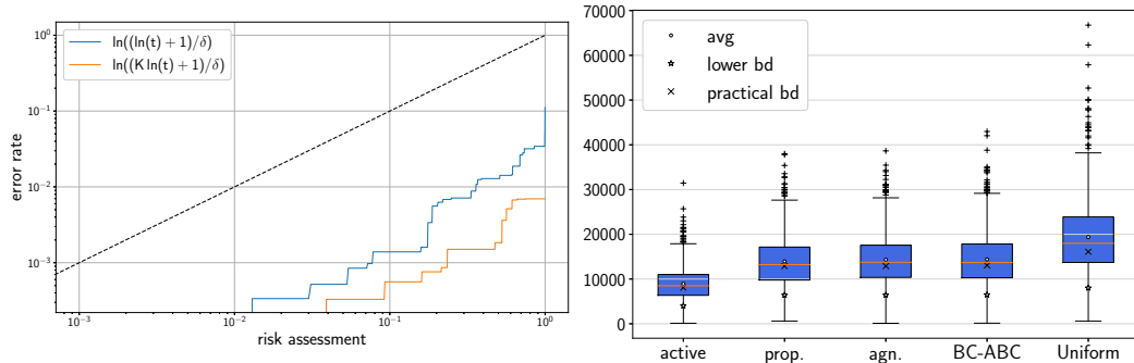
Figure 2: (Left) Risk assessment calibration on a log-log scale. (Right) Stopping time boxplot for \mu = [0.1 \ 0.4 \ 0.3; 0.2 \ 0.5 \ 0.2; 0.5 \ 0.1 \ 0.1] \in [0, 1]^{(K+1) \times J} when \beta = [1/3, 1/3, 1/3] , \alpha = [0.4, 0.5, 0.1] with Bernoulli distributions.
