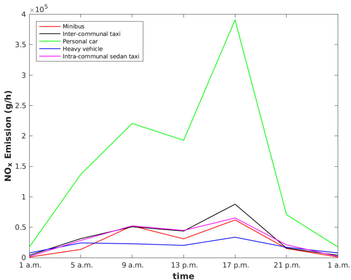
Figure 8. Total vehicle emission of \text{NO}_x for different vehicle types in Yopougon.
