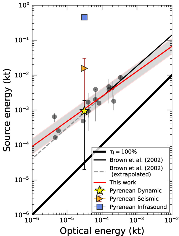
Figure 13. Energy calibrations of well-known bolides around the ton-scale TNT. For further details about the background data, see Fig. 12. The Pyrenean impact energy is displayed as the result of dynamic, seismic, and infrasound methods along with associated uncertainties. The best fit uncertainty (grey area) represents the standard deviation of the calibrated bolides.
