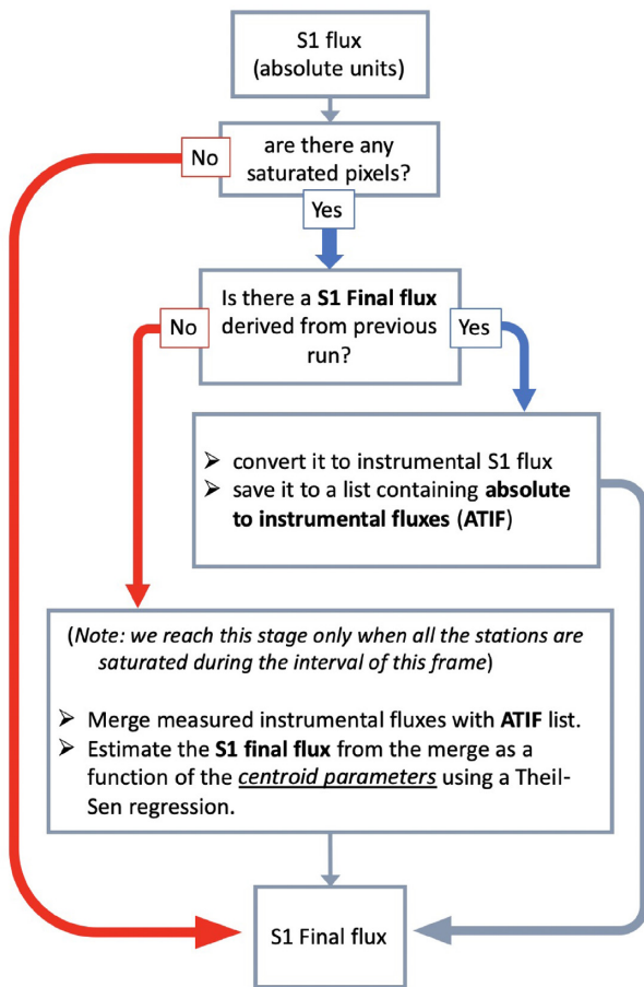
Figure A2. Map of the second run through the data. This will be applied as the first run, to all the frames from all stations. For the few segments where all the stations are saturated it is necessary to obtain a best flux fit on centroid parameters for each station, and assign weights on the final flux for those less saturated. The last step is to run a weighted mean through the final flux from all the stations to obtain the final light curve. The routines are developed in PYTHON open source programming language.
