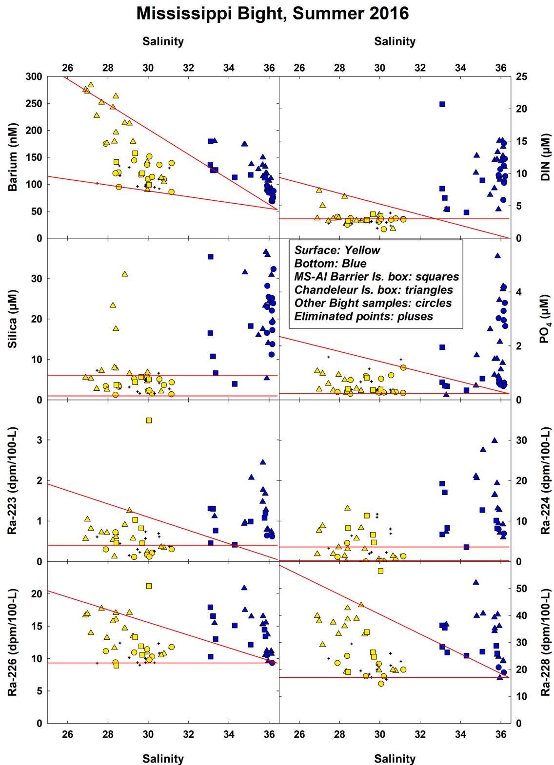
Fig. 4. Dissolved barium (Ba), dissolved inorganic nitrogen (DIN), dissolved silicic acid (DSi), dissolved inorganic phosphorus (DIP) concentrations, and Ra activities ( 223 Ra, 224 Ra, 228 Ra, 226 Ra) as a function of salinity in Mississippi Bight surface (yellow) and bottom (blue) waters in summer 2016. Extrapolations of surface concentration versus salinity to zero salinity are shown in red, and represent trends to high and low estimates of “effective” river concentrations (C*; see also Supplementary Table S1). (For interpretation of the references to colour in this figure legend, the reader is referred to the web version of this article.)
