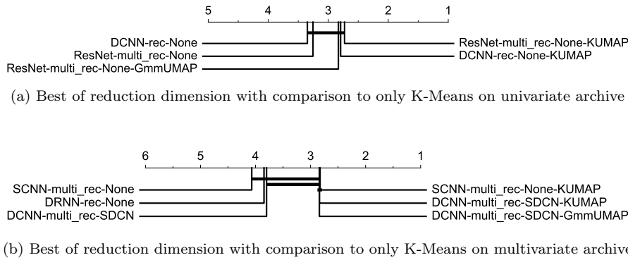
Fig. 13 Comparison clustering performance performed either directly on the learnt representation or after a dimension reduction (UMAP) with different clustering methods (GMM an K-Means) with NMI measure.
