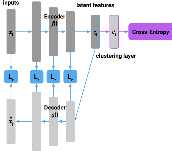
Fig. 7 DEPICT method: The DNN is trained to both reconstruct the data at each layer depth and obtain better confidence into predicting clustering pseudo labels with cross-Entropy.
