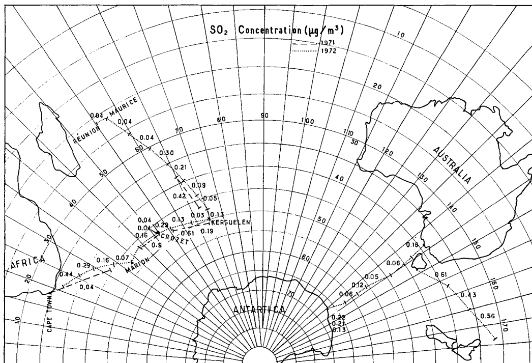
Fig. 6. \text{SO}_2 atmospheric concentration over Subantarctic and Antarctic areas
