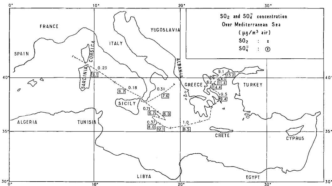
Fig. 5. \text{SO}_2 and \text{SO}_4 atmospheric concentrations over Mediterranean Sea
