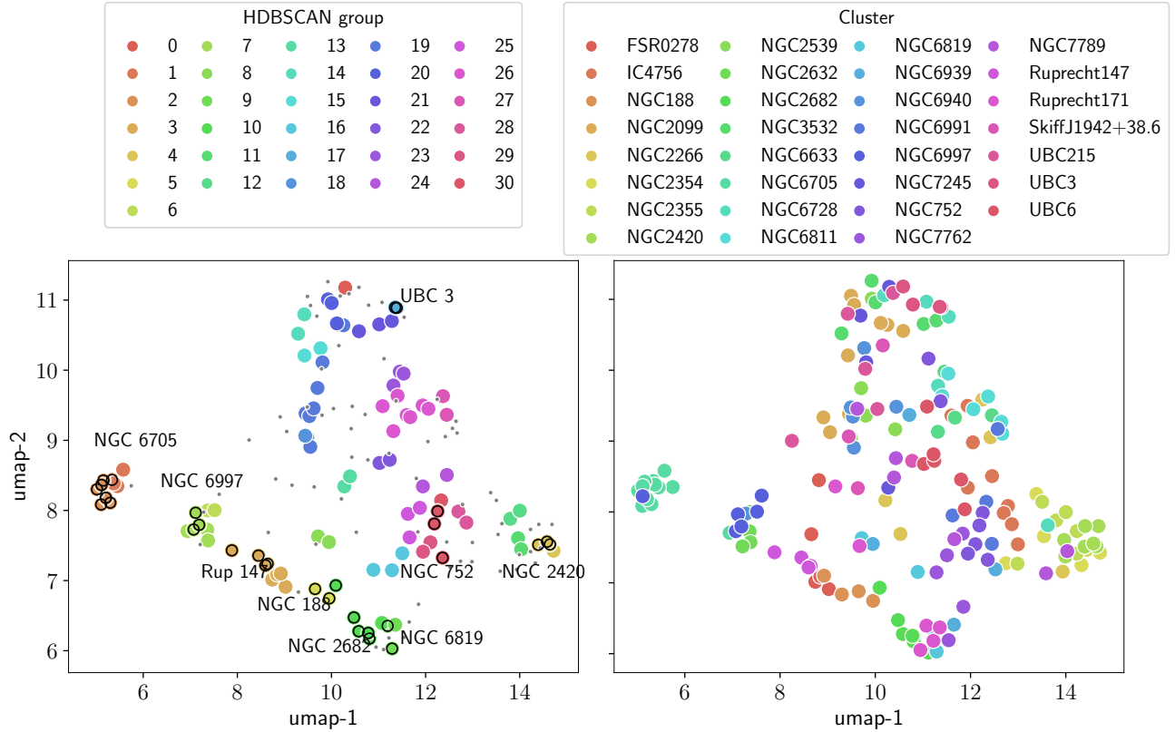
Fig. 5. UMAP projections of the stars in the high-precision sample. The groups are coloured according to whether they were found by HDBSCAN ( left ) or are real clusters ( right ). The grey points correspond to stars that were found as noise. The stars highlighted with black circles were recovered in a group with at least 40% homogeneity and completeness (those in boldface in Table 2), and the corresponding cluster is labelled.
