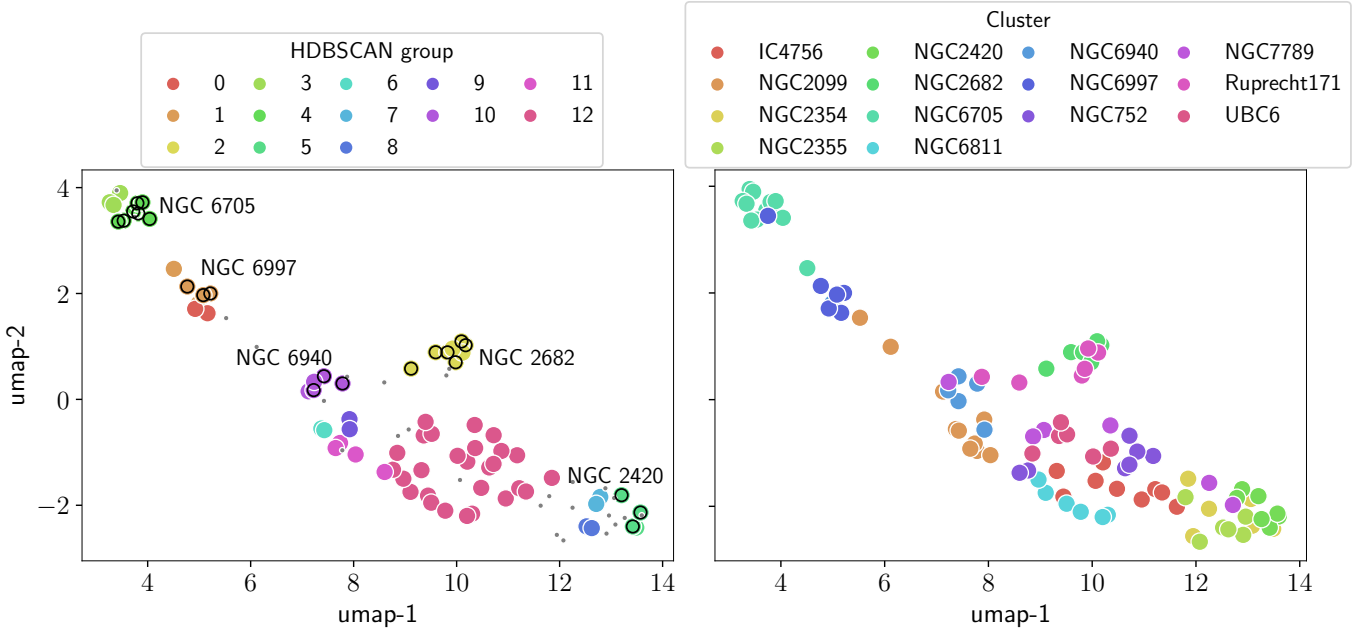
Fig. 6. Similar to Fig. 5 but only using clusters with at least 6 members in the high precision sample. UMAP projections of the stars colouring the real clusters ( right ), and the groups found by HDBSCAN ( left ). The stars highlighted in black circles are those recovered in a group with at least 40% homogeneity and completeness (those in boldface in Table 3).
