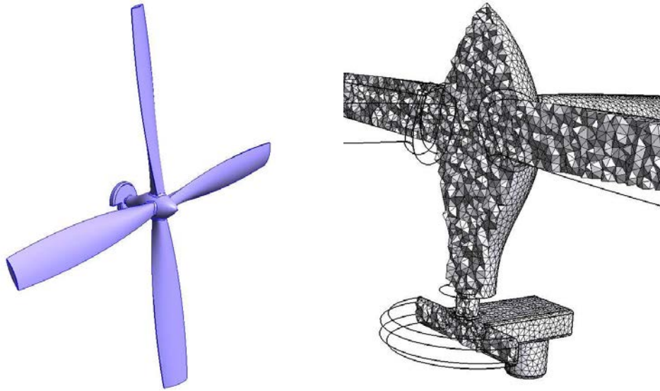
Figure 4. CAD model of a propeller (left) and its volume mesh (right)
