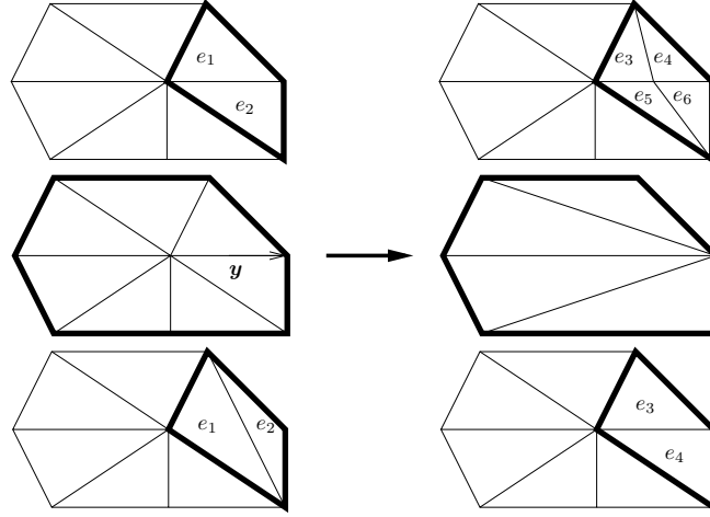
Fig. 2. Local mesh modifications. Edge split (top), edge collapse (middle) and edge swap (bottom). The zone depicted in bold represents the cavity that is modified by the local mesh modification.
