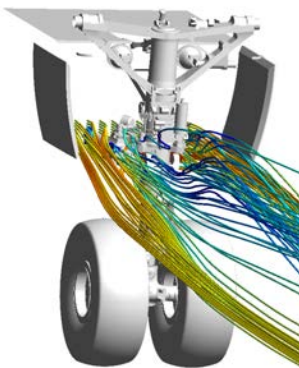
streamlines (P. Geuzaine, Cenaero)
