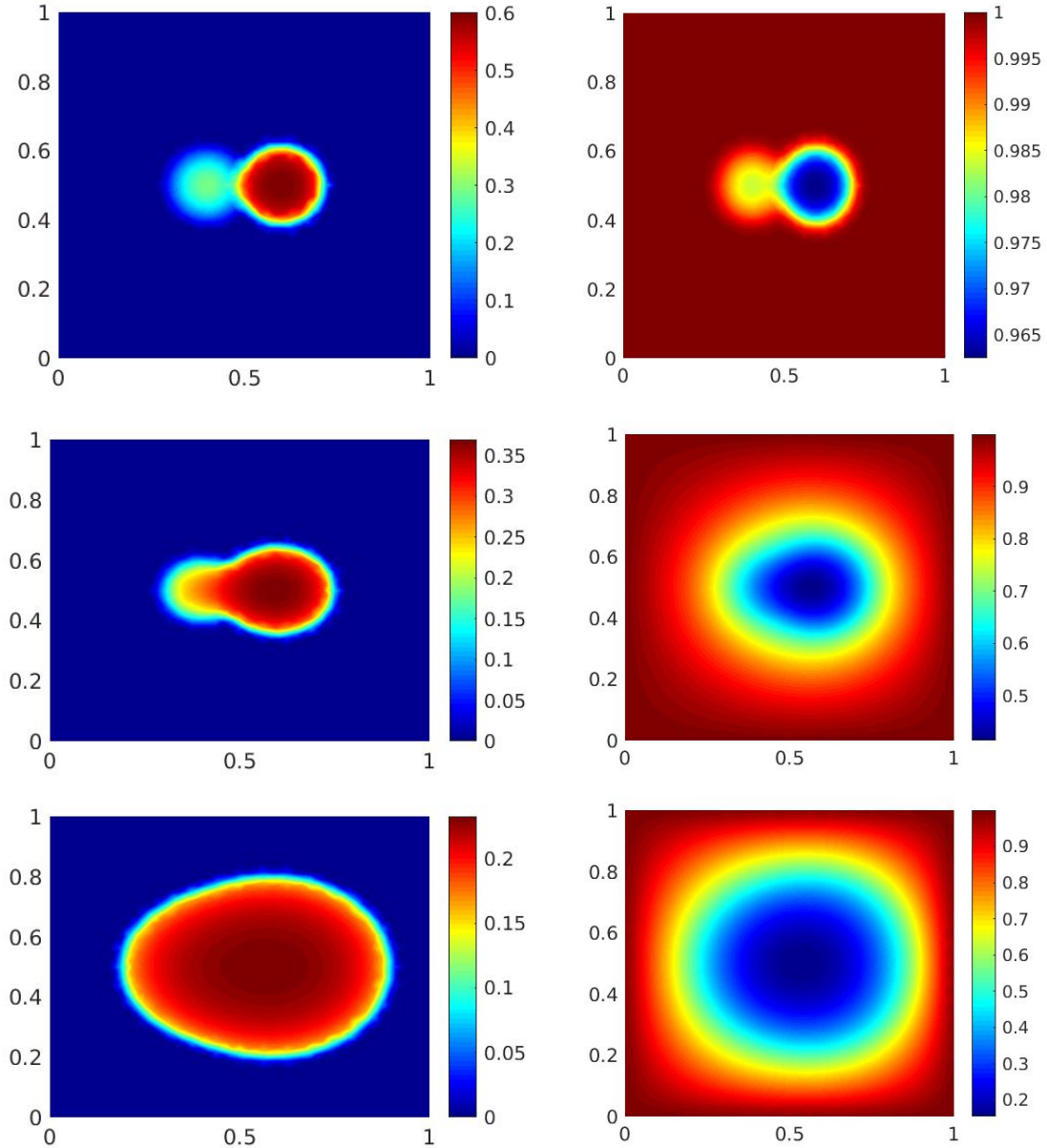
FIGURE 2. Test case 2: Evolution of M (left column) and S (right column) for t = 10^{-4} (top row), t = 10^{-2} (middle row) and t = 2 (bottom row).
