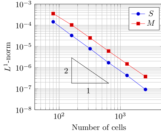
FIGURE 1. Test case 1: L^1 norm of the error between the reference solution and the solutions computed on coarser grids at final time T = 10^{-3} .
