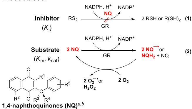
Scheme 1. Redox-Active 1,4-Naphthoquinones as Subversive Substrates of NADPH-Dependent Disulfide Reductases.
