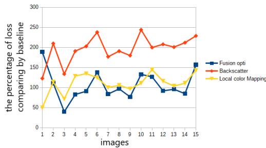
Fig. 9: Percentage of loss with Fusion Optimize
