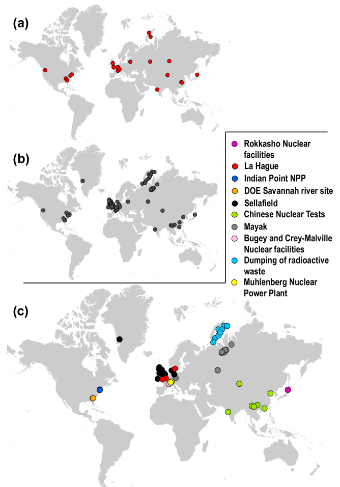
Figure 5. ^{137}\text{Cs} activity levels attributed to local and regional radioactive releases. (a) Local and regional sources identified in the literature. (b) Releases associated with these events detected in sediment cores. (c) Some examples of events detected in sediment cores.
