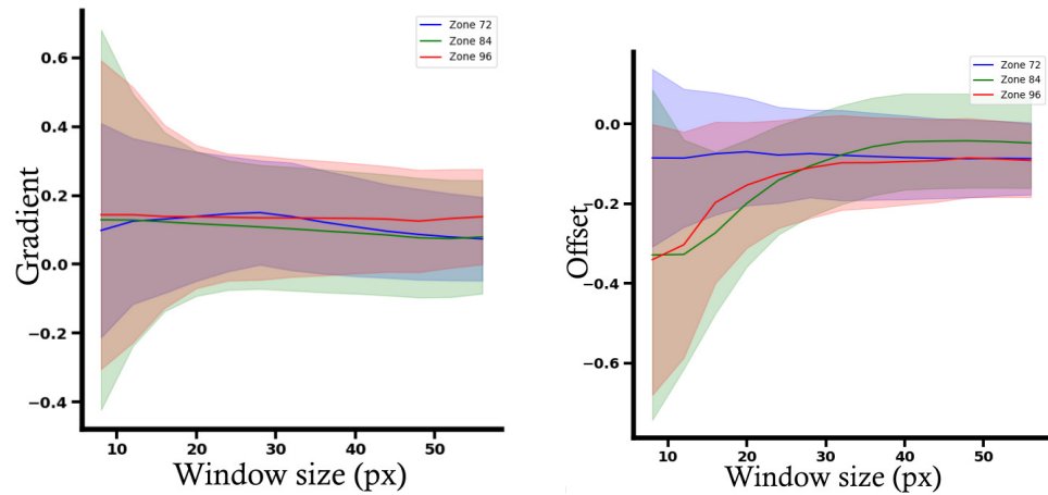
Figure 3 Convergence of the gradient and offset of circumferential deformations as a function of window size in the “sensitive” areas.
