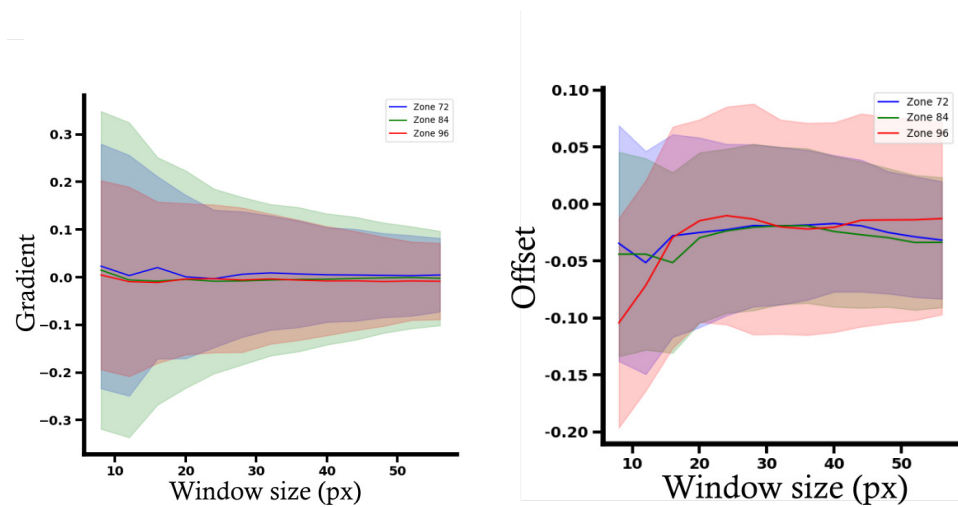
Figure 4 Convergence of the gradient and offset of radial deformations as a function of window size in the “sensitive” areas.
