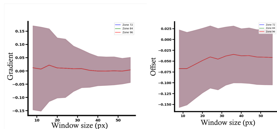
Figure 2 Convergence of the gradient and offset of radial strains as a function of window size across the AF on average.
