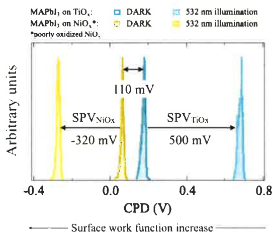
Fig. 3 Normalized histograms extracted from CPD maps showing distributions of CPD values on top of the TiO x and NiO x sides for the LHM with poorly oxidized NiO x .
