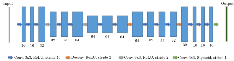
Fig. 2: Network architecture.
