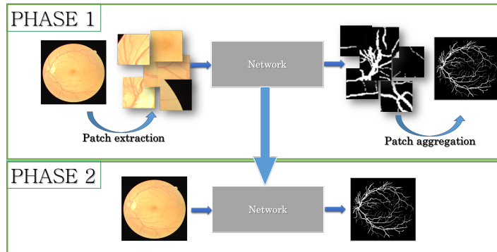
Fig. 1: The proposed framework. Phase 1: The network is fed with patches extracted from the original images. Phase 2: The network is fine-tuned with the full sized images.
