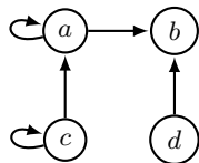
Fig. 1: AG showing that Reinforcement and Strong Self-Contradiction are incompatible.
